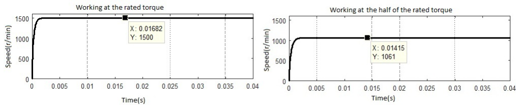
Figure 7: Speed of the motor with different value of torque
