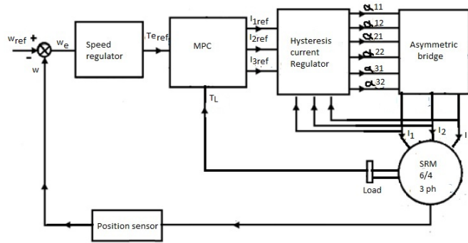
Figure 3: Control strategy
