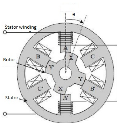
Figure 1: A three phase structure of the SRM
