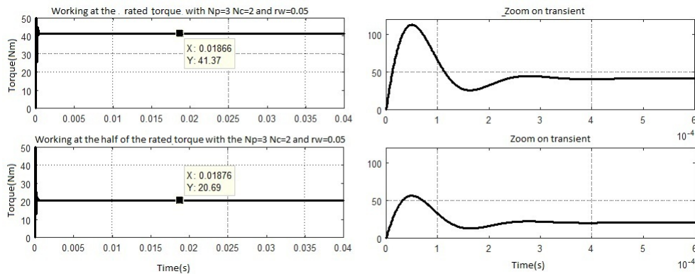
Figure 6: Torque control
