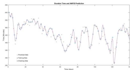
Figure 5: Results of the Prediction Using ANFIS for Duration Time.
