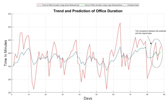
Figure 4: Trend and Prediction of Occupying an Office Using EWMA.
