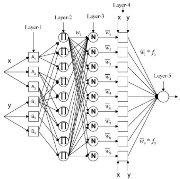
Figure 1: ANFIS Architecture Example.
