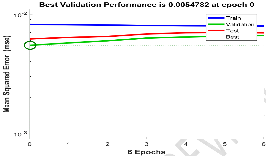
Fig 2. Model 1: the feed forward back propagation algorithm with training function was TRAINRP and the adaptive learning function is LEARNMGD the MSE is 0.00547823.
