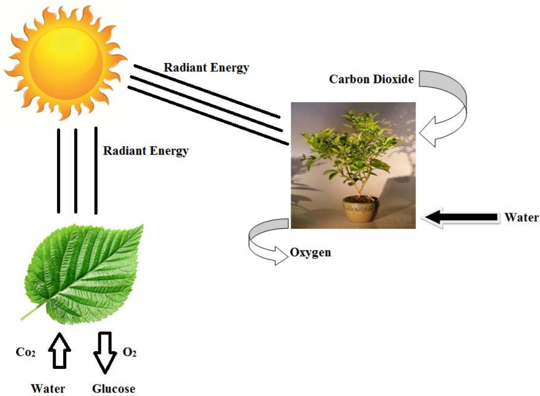
Fig.1. Picture representation of Photosynthesis process
