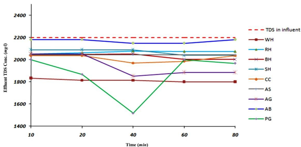
Figure 4. Changes in TDS concentration for different adsorbent material
