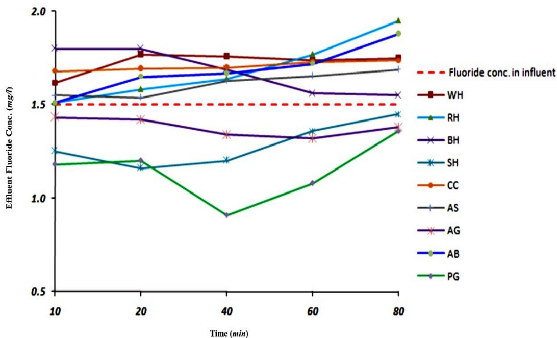
Figure 3. Changes in Fluoride concentration for different adsorbent material.
