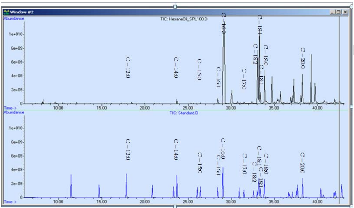
Fig. 1: Fatty acid methyl ester chromatogram against FAME standard
