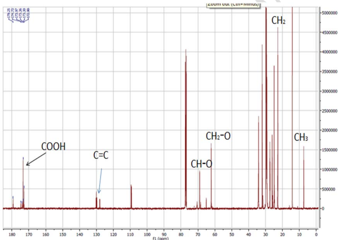
148 149 Figure 4: ^{13}\text{C} -NMR spectrum of Pachira aquatica seed oil.
