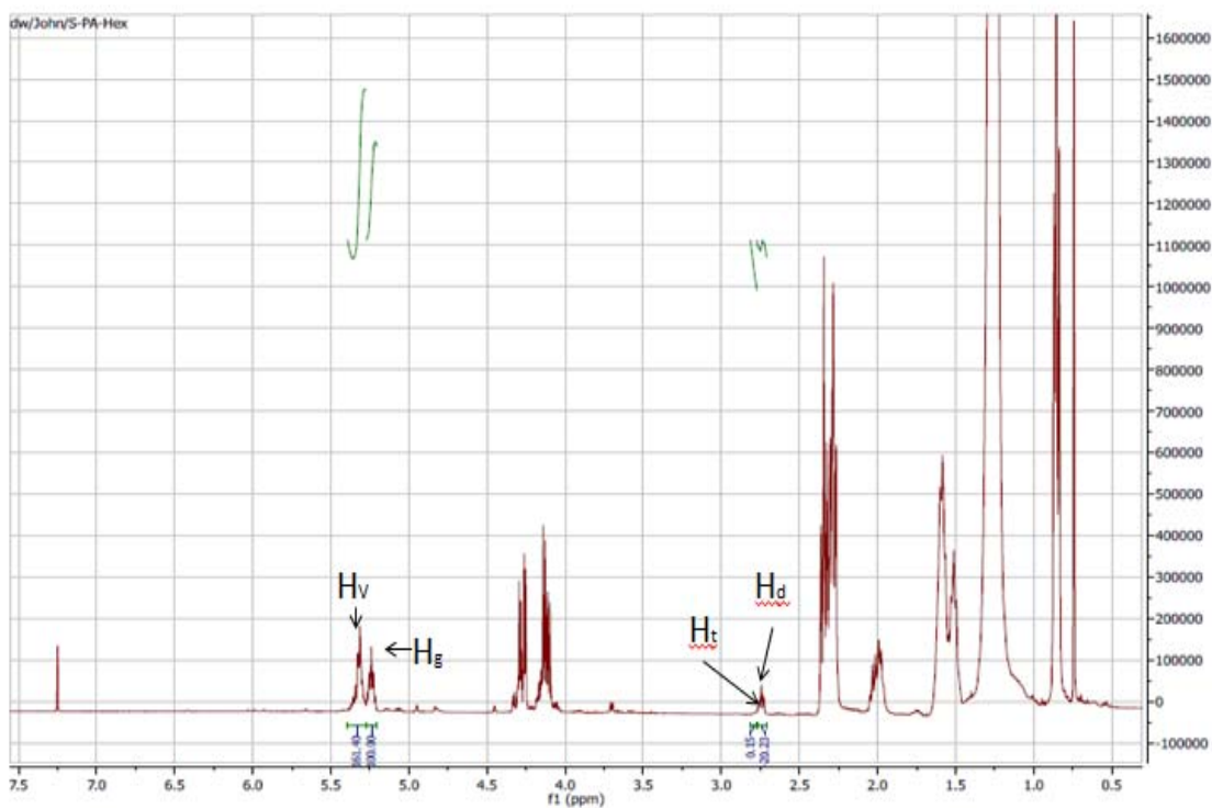
Figure 2: ^1\text{H} NMR spectrum of Pachira aquatica seed oil.
