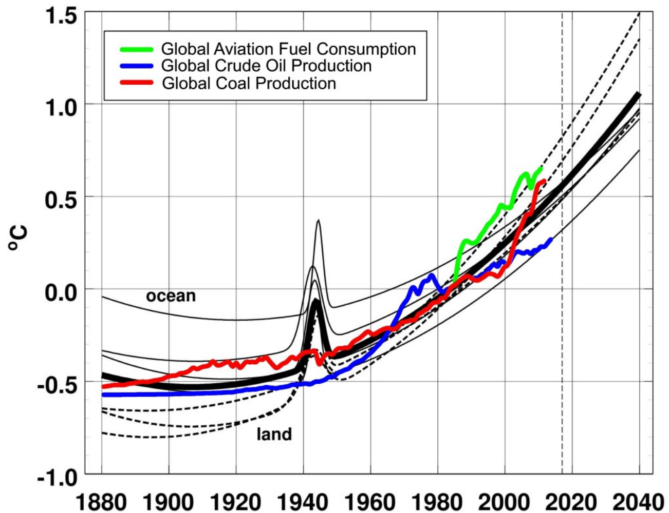
Fig. 2. Copy of Gottschalk's fitted curves for eight NOAA data sets showing relative temperature profiles over time [15] to which are added proxies for particulate pollution. Dashed line: land; light line: ocean; bold line: weighted average. From [11].
