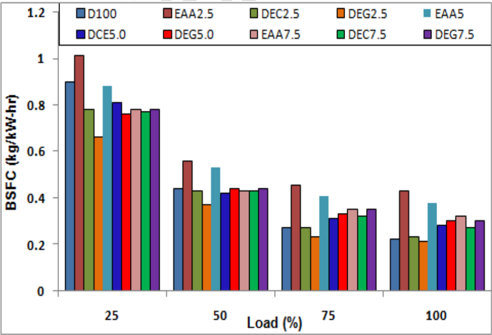
Fig.4 BSFC variation of blend fuels with Load
