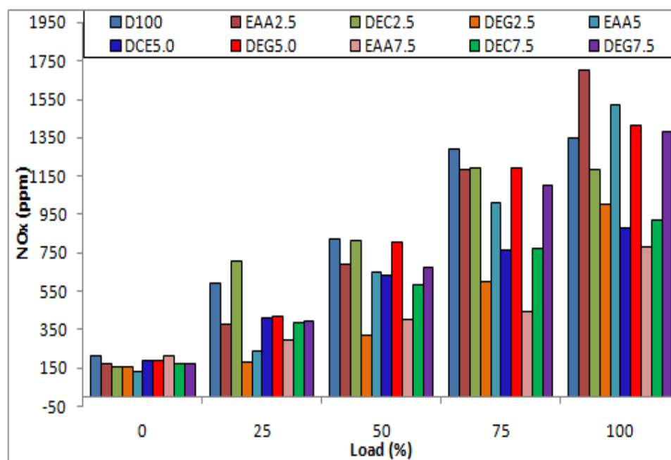
Fig. 6 NO x variation of blend fuels with Load
