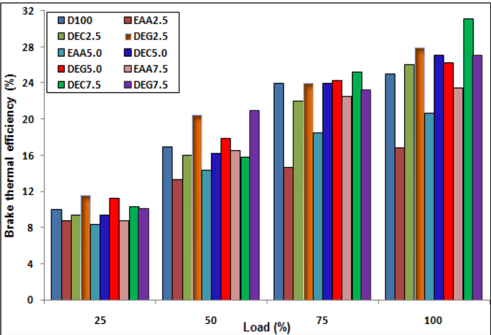
Fig.3 Thermal efficiency variation of blend fuels with Load
