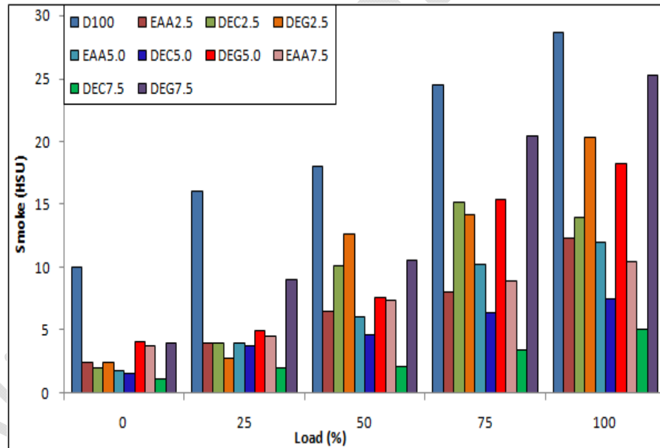
Fig. 5 Smoke variation blend fuels with Load
