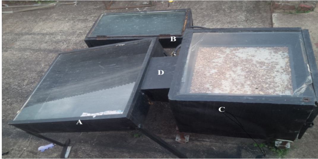
Fig i: The Experimental Solar Dryer
