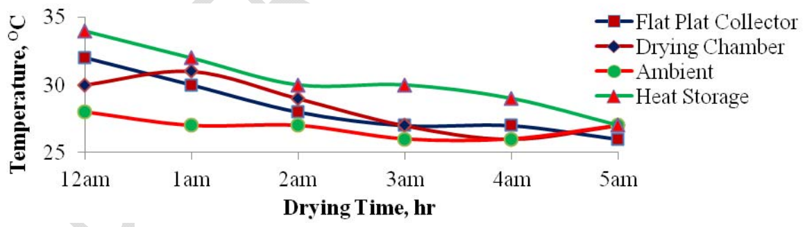
Fig vi: Temperature of solar dryer parts when (a) collector covered and valve opened (b) collector covered and valve closed (c) collector uncovered and valve opened (d) collector uncovered and valve closed at night
