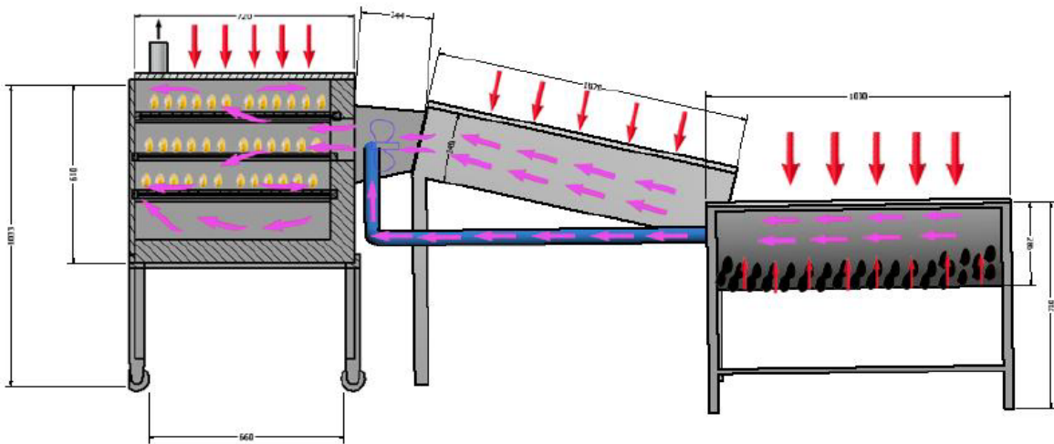
Figure iv: Diagram showing the heat source and airflow direction inside the dryer at night
