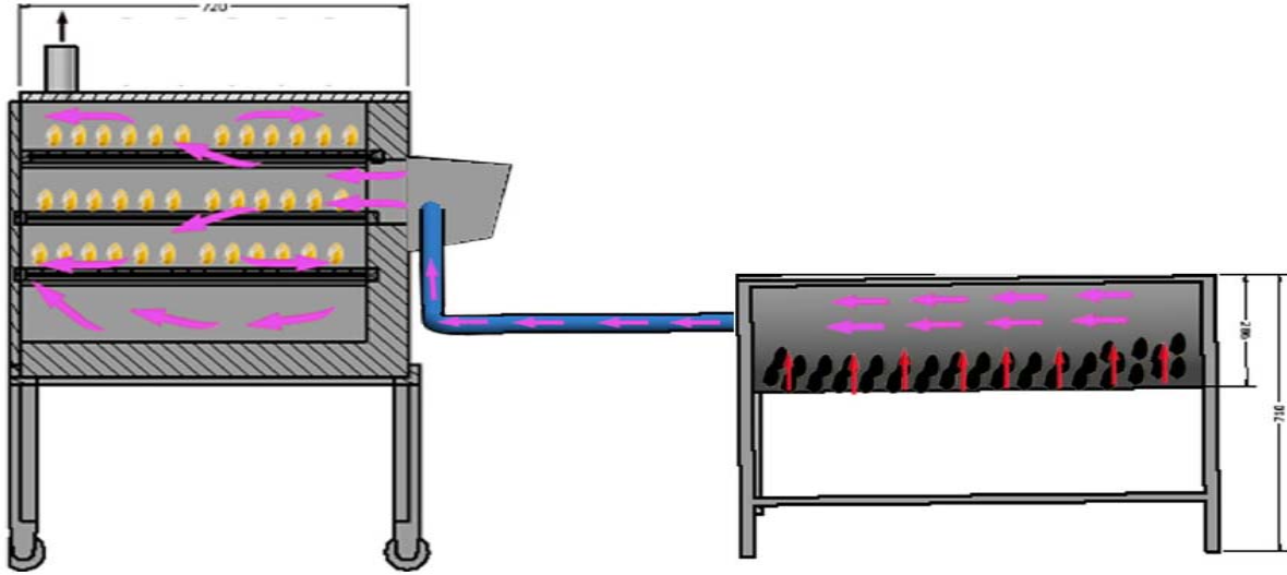
Figure iv: Diagram showing the heat source and airflow direction inside the dryer at night
