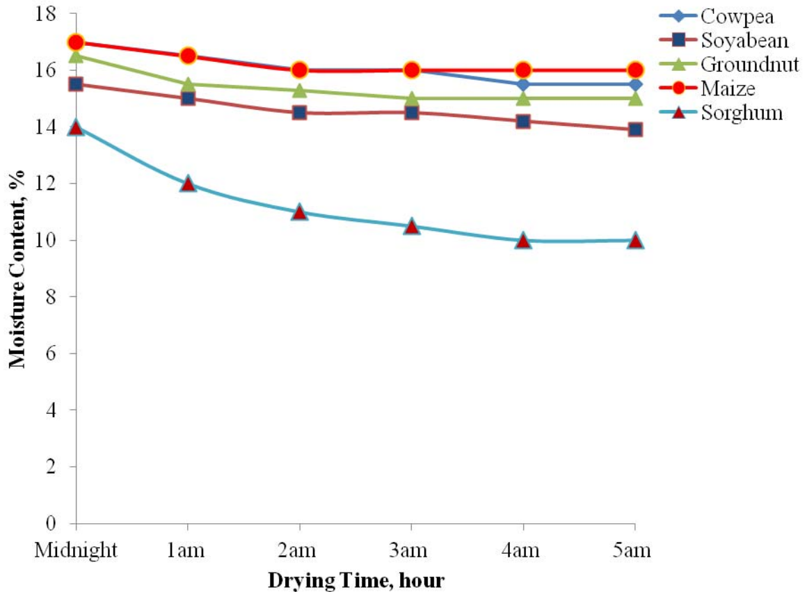
Figure vii: Variation in Moisture Content of Grains Using the Solar Dryer at Night
