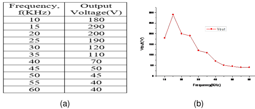
Figure 9: (a) Corresponding values of Frequency vs output voltage, and (b) The output characteristics of power transformer (Frequency vs output voltage).
