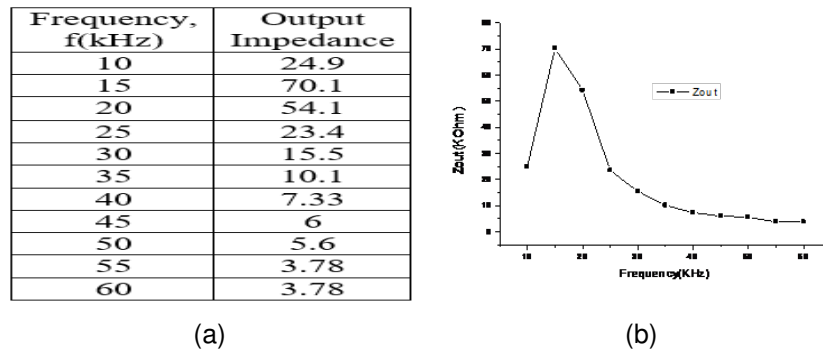
Figure 10: (a) Corresponding values of Frequency vs output impedance, and (b) Frequency vs output impedance characteristics of the input coupling.
