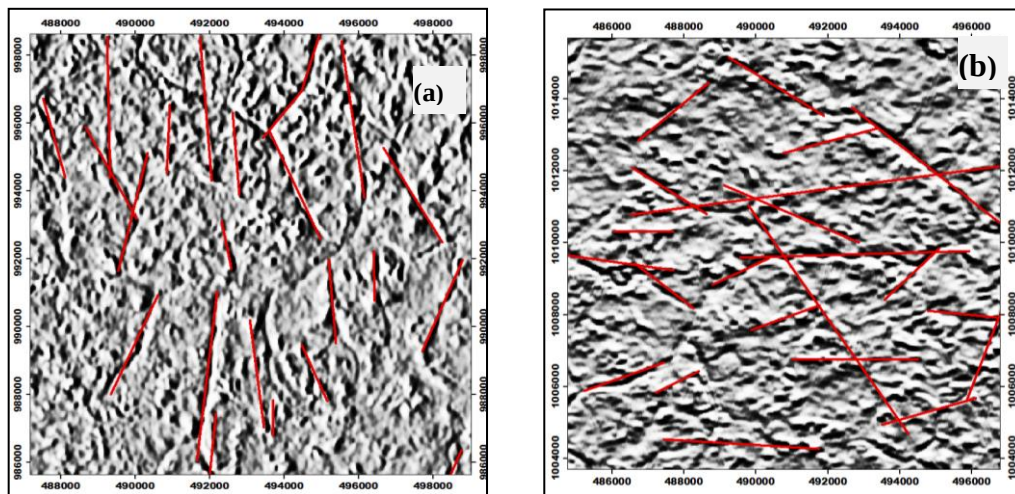
Figure 2: identification of the lineaments on filtered images (a) filters of Sobel E-SW enhanced the lineaments NS on CP1 234 ; (b); filter of Yésou enhanced the lineaments.
