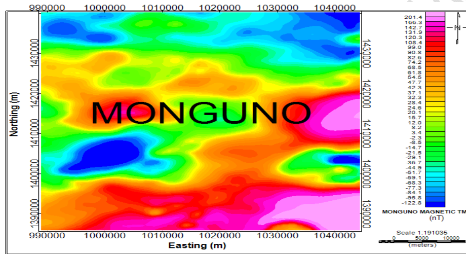
Fig. 2: Total magnetic intensity map
