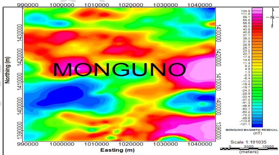
Fig.3: Residual magnetic map
