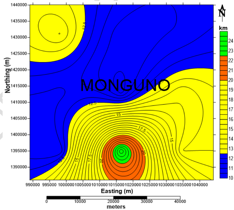
Fig. 4: Curie Depth map (contour interval of 0.5km).
