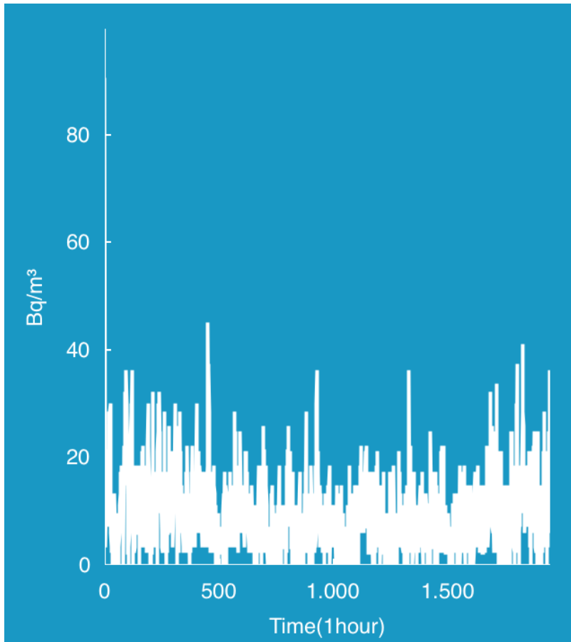
Fig. 5 – Monitoring of 1943 hour series from RD200 in ITA and ACA Tower using (Bq/m 3 ) unit.
