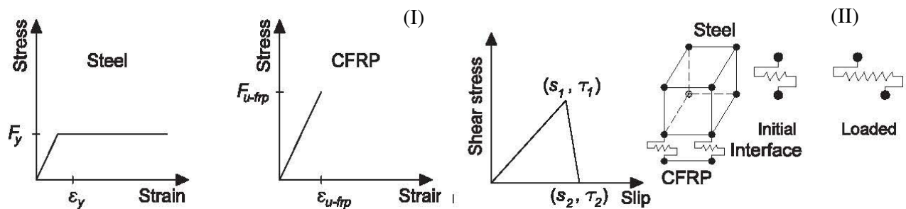
FIG. 2 Material modeling (I) Constitutive behavior of Steel and CFRP, (II) Interface element model
