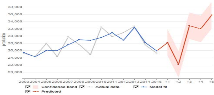
432 433 Fig.7:Actual value, fitted value and forecast value and confidence band in GMDH model 434
