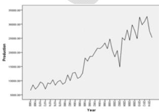
Fig 2. Time series plots of oilseeds
