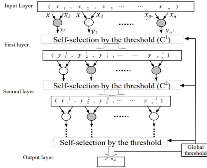
Figure (Fig.) 1: Structure of the GMDH algorithm.
