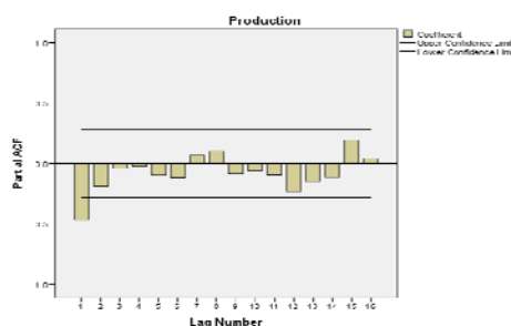
Fig.6: PACF of 1 st differenced series by lag
