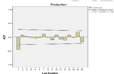
Fig. 5: ACF of 1 st differenced series by lag
