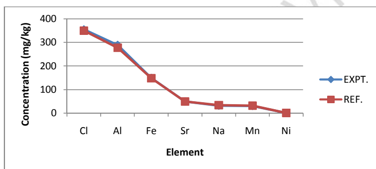
Fig. 6. Experimental and reference values for cabbages IAEA 359.
