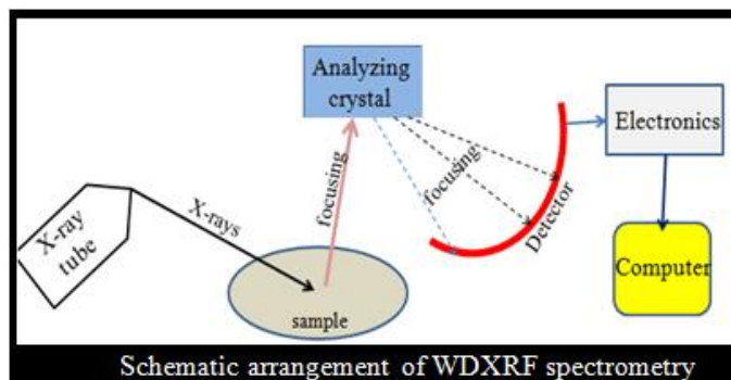
Fig. 4. Schematic arrangement of WDXRF spectrometer.
