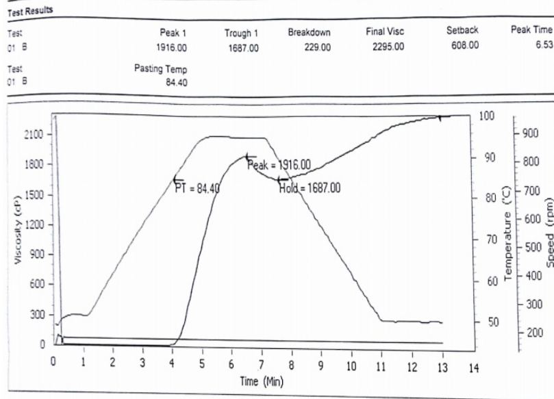
Figure 2: Pasting properties of Blend B (80% Unripe plantain, 34% Soybean and 6% Ginger)
