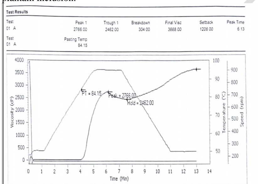
Figure 1: Pasting properties of Blend A (100% Unripe Plantain)
