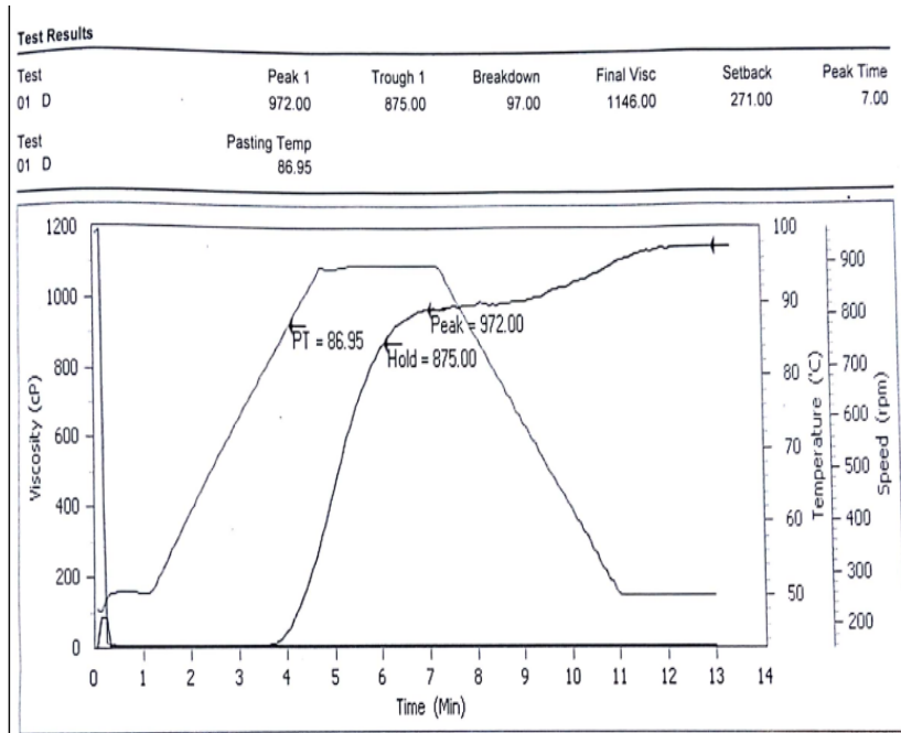
Figure 4: Pasting properties of Blend D (60% Unripe Plantain, 38% Soybean and 2% Ginger)
