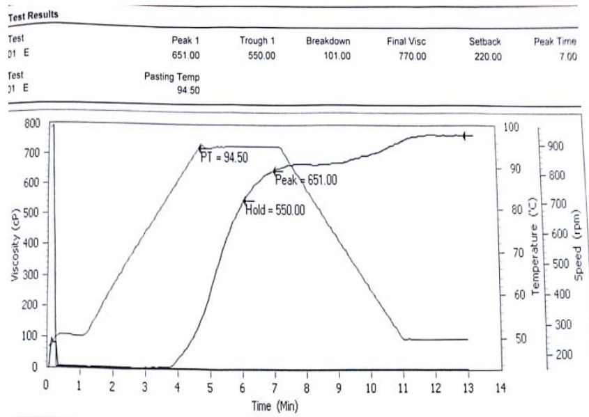
Figure 5: Pasting properties of Blend E (50% unripe plantain: 50% soybean)
