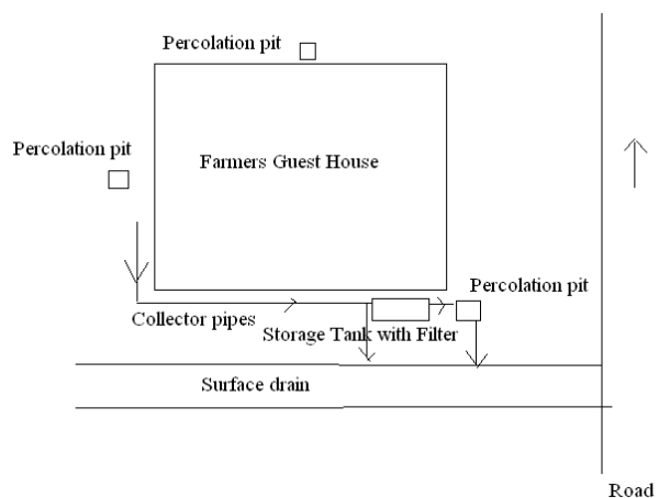
Fig. 1: schematic diagram of rooftop water harvesting system
