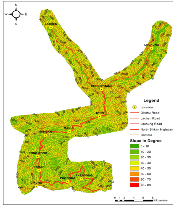
Fig. 2. Slope map of the study area
