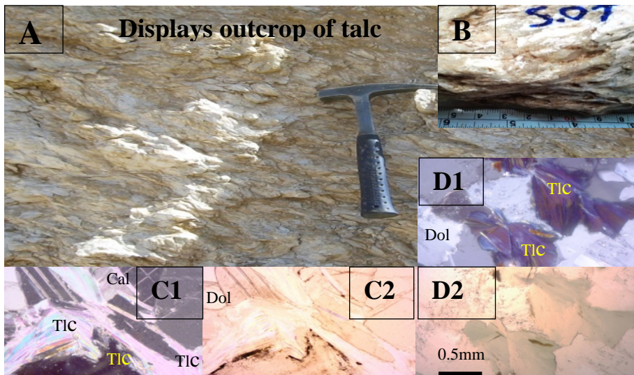
Plate (A) shows an exposure abandoned or quarry talc' schist into local mine in central of the study area. (B) Shows a hand specimen of talc. (C1, C2, D1 & D2) Showing the photos microscope of talc schist which composed minerals of talc, calcite and dolomite. (C1 & D1) taken under the cross Nicole microscope, but (C2 & D2) under plain polarizing light.
