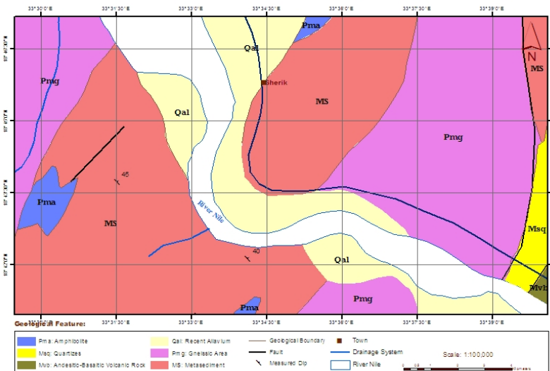
Figure :( 3) Regional geological map of the study area, complied by Geological Research Authority of the Sudan, and Robertson Research, 1988.
