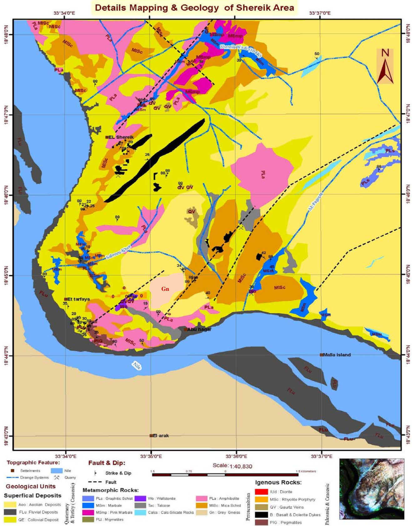
Fig.4.1. Detailed geological map of emphasizing structures of the El Sherek study area east Nile bank.
