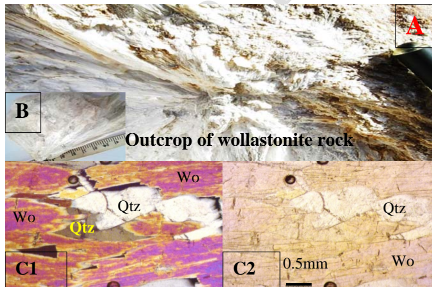
Plate (A Explains wollastonite rock into a local quarry south mapped area. (B) Showing a hand specimen of wollastonite rock. (C1 & C2) explained the photo-microscope of wollastonite skarn, rocks, radiated shape, mainly consisting of wollastonite and little quartz. (C1) Taken in cross Nicole and (C2) in the plain polarizing light.
