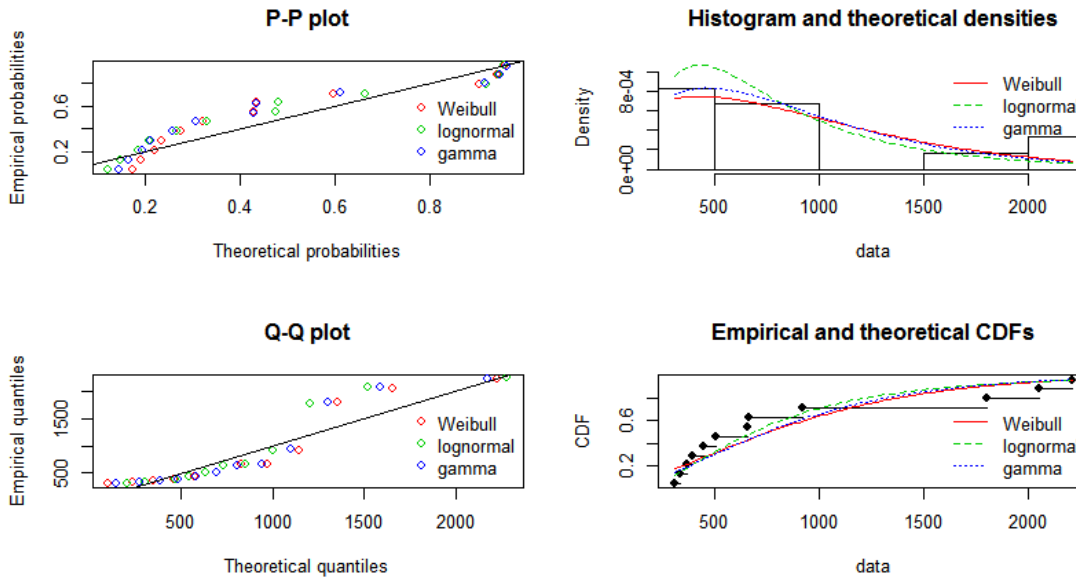
Figure 6 b: Four Goodness-of-fit plots for various distributions fitted to continuous data (Weibull, gamma and lognormal distribution)
