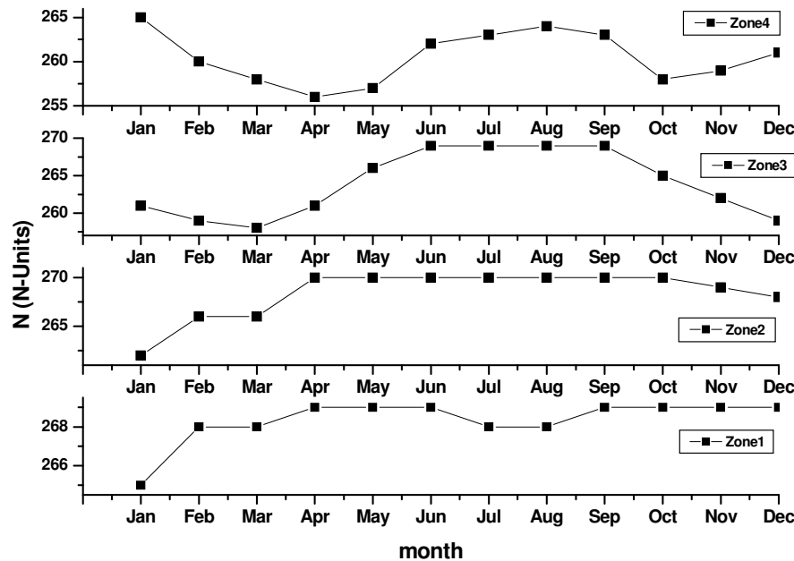
Figure 2: Seasonal Variation of Surface Refractivity (N) at 10 m for different Climatic Zones across West Africa (1983 – 2005)
