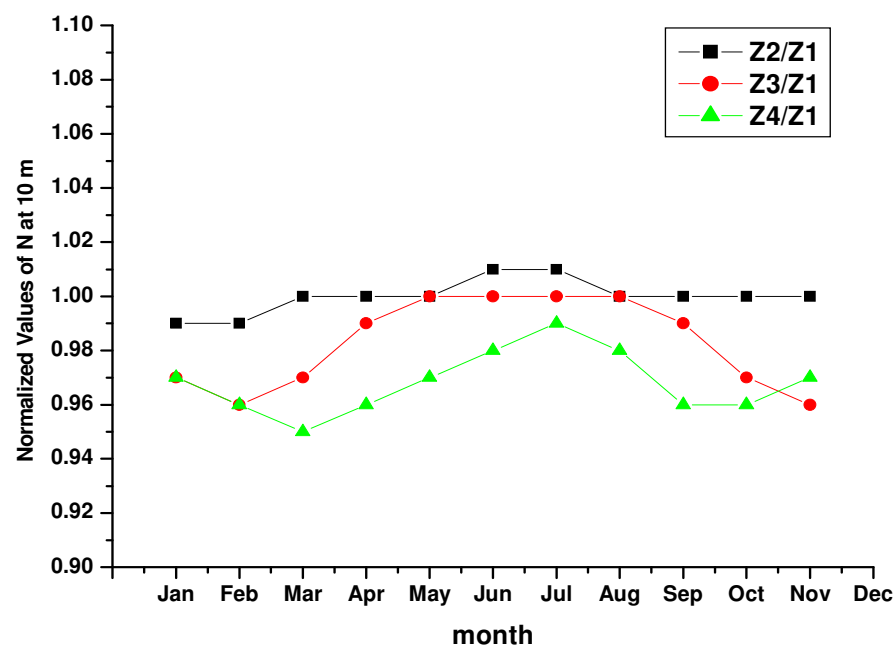
Figure 4: Monthly Averaged Normalized Values of Surface Refractivity Index at 10 m across different Climatic Zones in West Africa (1983 – 2005)
