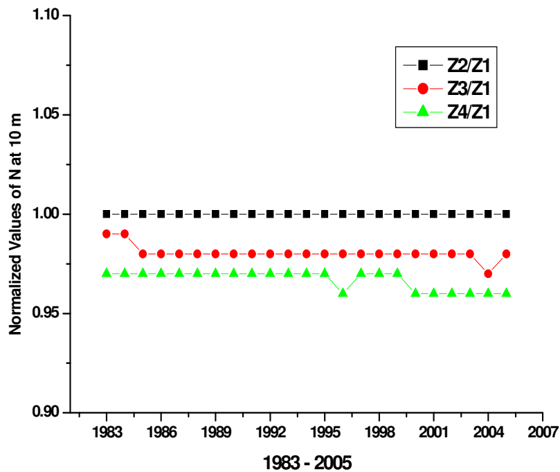
Figure 6: Annual Averaged Normalized Values of Surface Refractivity Index at 10 m across different Climatic Zones in West Africa (1983 – 2005)
