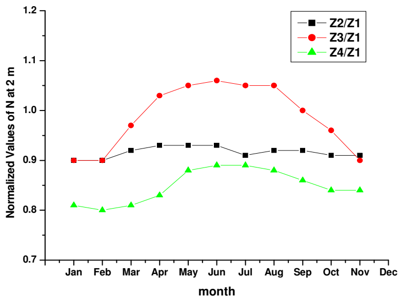
Figure 3: Monthly Averaged Normalized Values of Surface Refractivity Index at 2 m across different Climatic Zones in West Africa (1983 – 2005)
