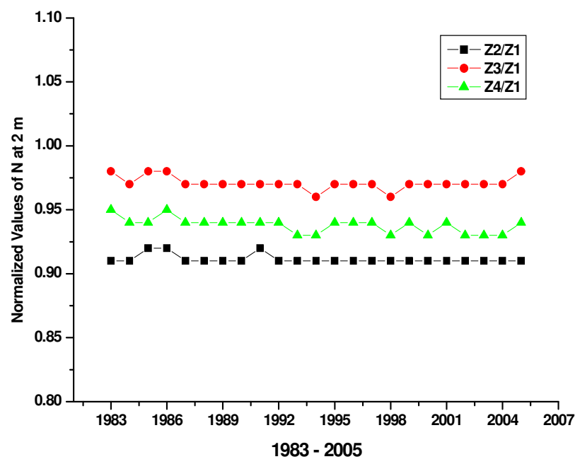
Figure 5: Annual Averaged Normalized Values of Surface Refractivity Index at 2 m across different Climatic Zones in West Africa (1983 – 2005)
