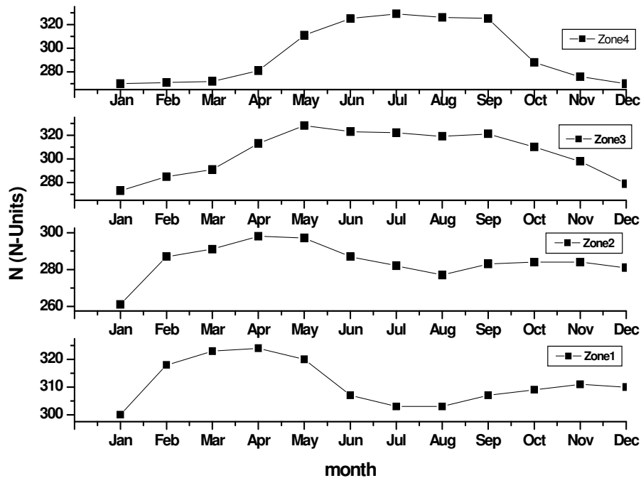
Figure 1: Seasonal Variation of Surface Refractivity (N) at 2 m for different Climatic Zones across West Africa (1983 – 2005)
