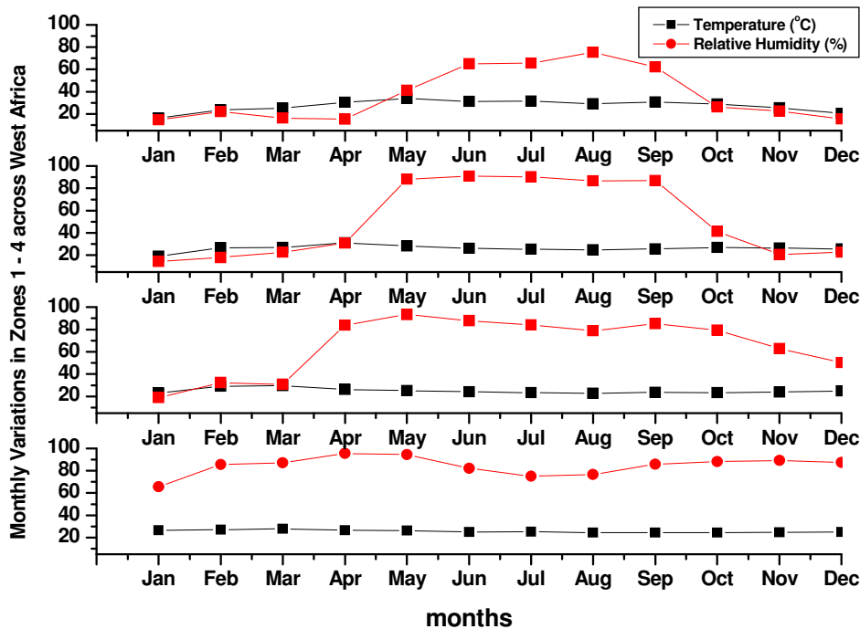
Figure 7: Seasonal Variation of Temperature and Relative Humidity in Different Climatic Zones across West Africa
