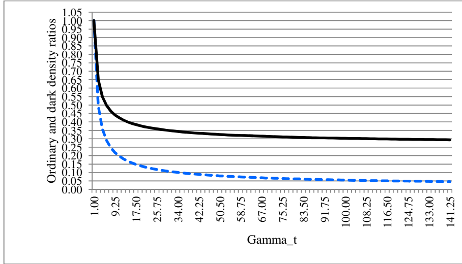
Figure 1: Decreasing trend of ordinary and dark matter density ratios
