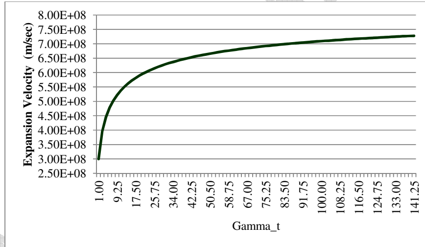
Figure 3: Increasing trend of cosmic expansion velocity
