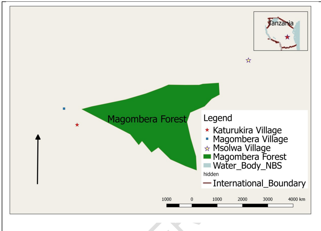
Figure 1. Map showing the Magombera Forest area was created using QGIS Version 2.18.15 with the help from Google Earth™
