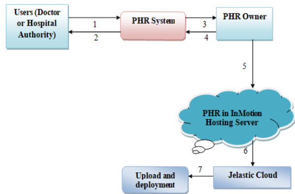
Figure 3: Architecture of PHR system
