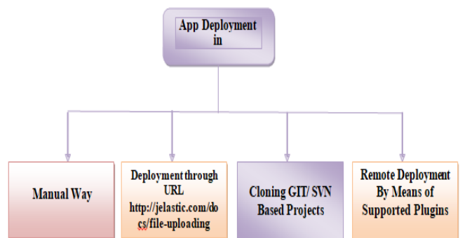
Figure 4: Jelastic ApplicationDeploymentMethods.
