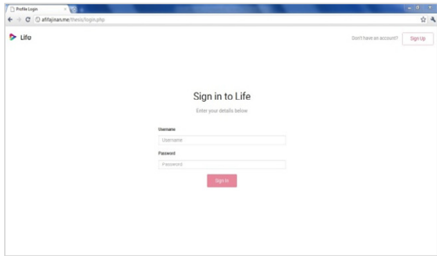
Figure 5: The LoginPage
