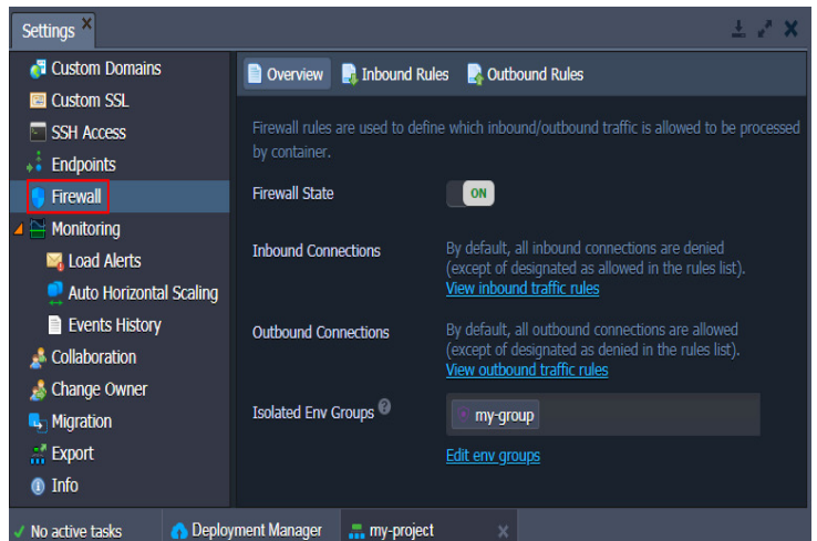
Figure 11: Option of inbound and outbound firewall rules.
