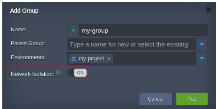
Figure 12: Option for create secure group in jelastc cloud.
