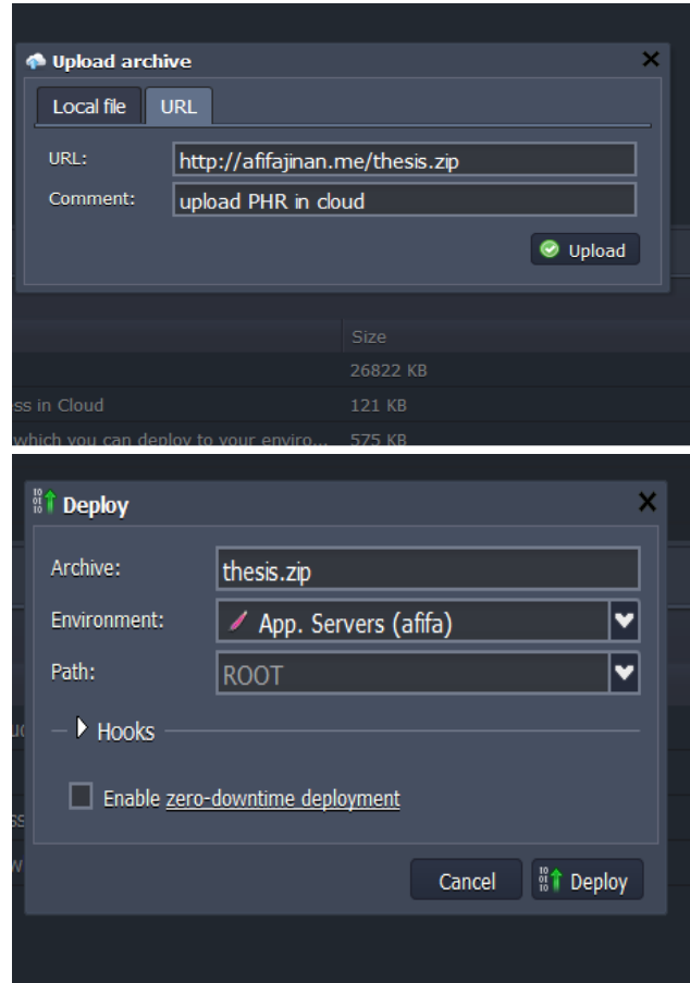
Figure 10: Uploading & Deploying PHR application in Jelastic CloudJiffy
