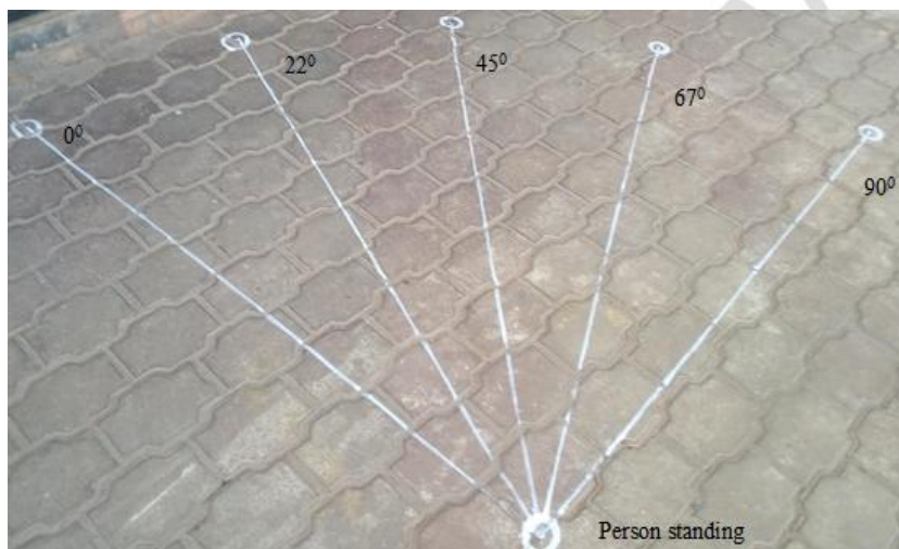
Figure 4. Marking angles using total station
