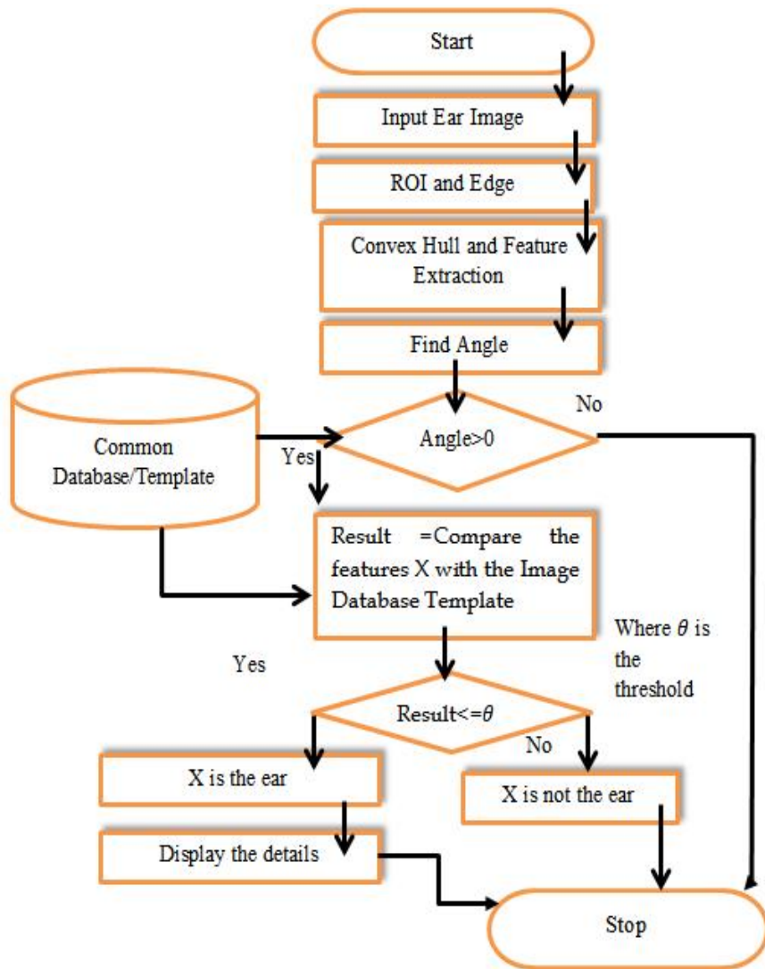
Figure 12. The general flow diagram of personal identification system
