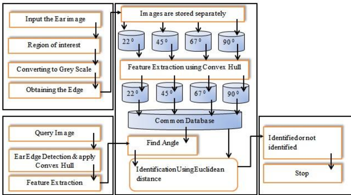
Figure 11. Flow chart of the system (Euclidean distance criteria)
