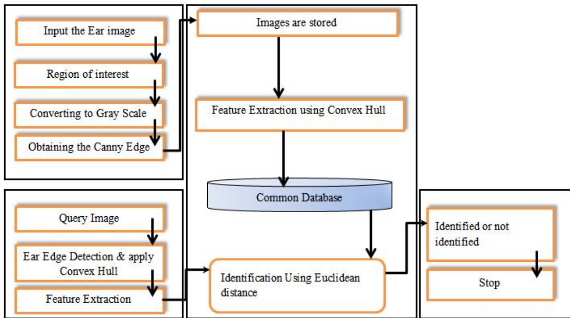
Figure 10. Flow chart for identification / matching process
