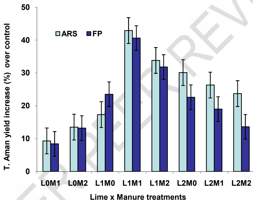
Fig. 3. Residual effects of lime and manure treatments on % grain yield (T. aman) increase over control at ARS and farmer's plot in Thakurgaon; results are the average of 2 years. L0, L1 and L2 represent lime dose at 0, 1 and 2 t ha -1 , respectively; M1 and M2 represent poultry manure and FYM, respectively.
