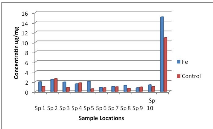
Figure 3: Concentration of iron across the sample points (Fe)
