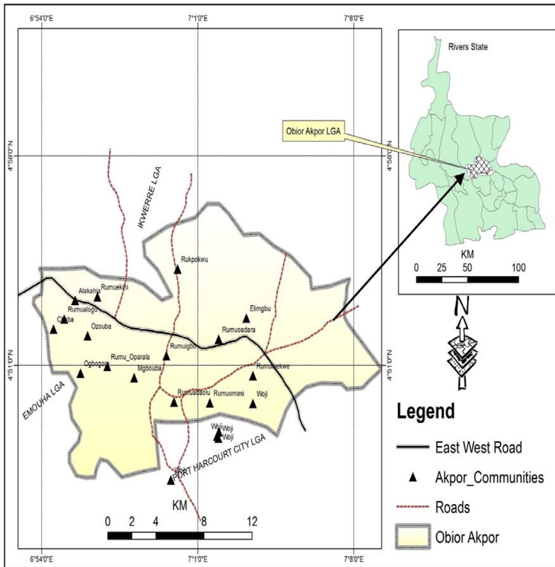
Figure 1: Study Area Showing the East West Road
