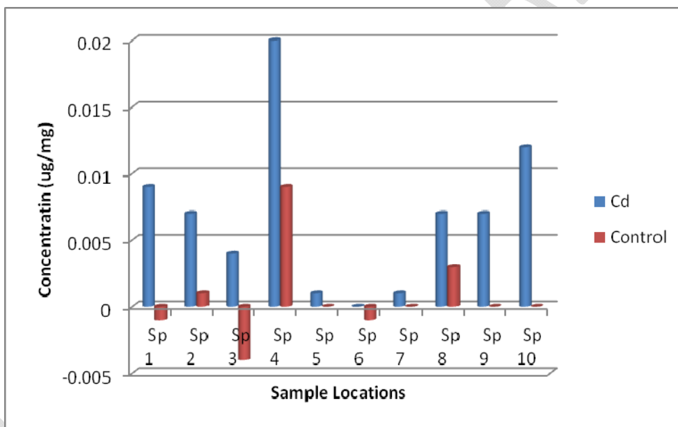
Figure 4: Concentration of Cadmium (Cd)
