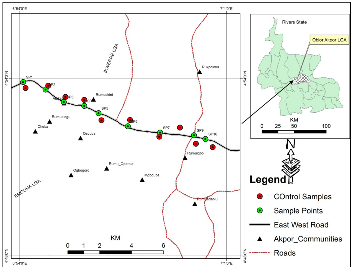
Figure 2: The East West Road in Obior/Akpor Local Government Area showing sampled points
