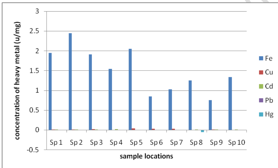
Figure 5: Distribution of heavy metals across the sample locations
