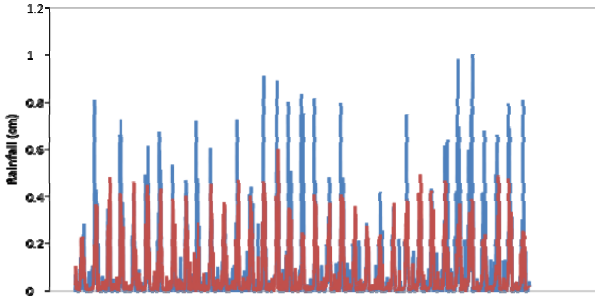
Fig 4: Feed forward back propagation algorithm with training function was TRAINLM and the adaptive learning function is LEARNGDM the MSE is 0.010077 (Model 4)
