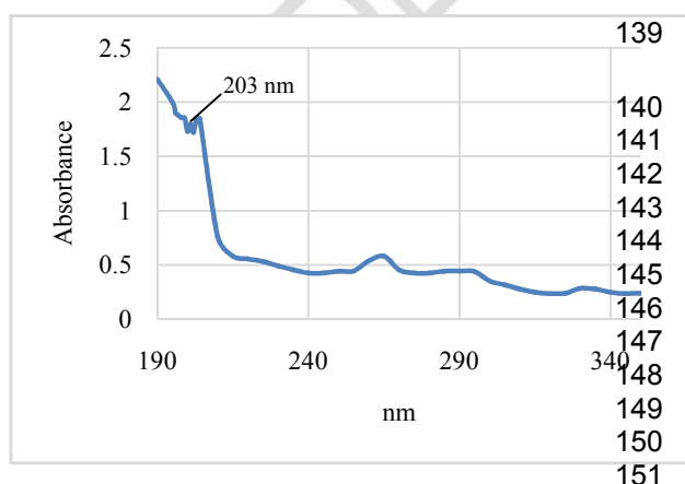
Figure 2. Wavelength scanning of SrO NPs as spectrophotometrically
