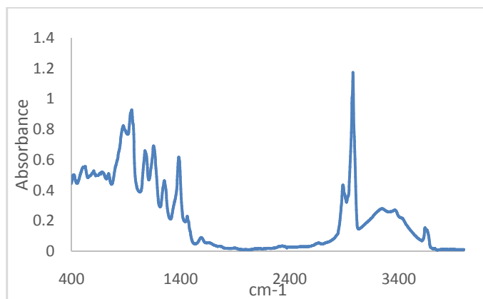
Figure 5. FTIR spectrum of SrO nanoparticles
