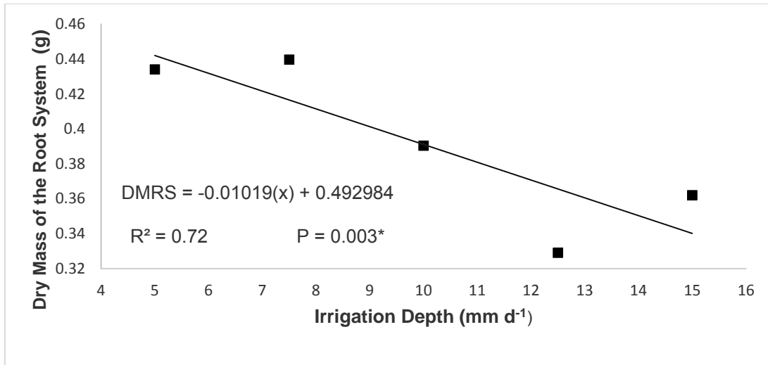
Fig. 4. Estimating the collecting dry mass of the root system (DMRS) of conilon coffee seedlings as a function of the irrigation depth.
