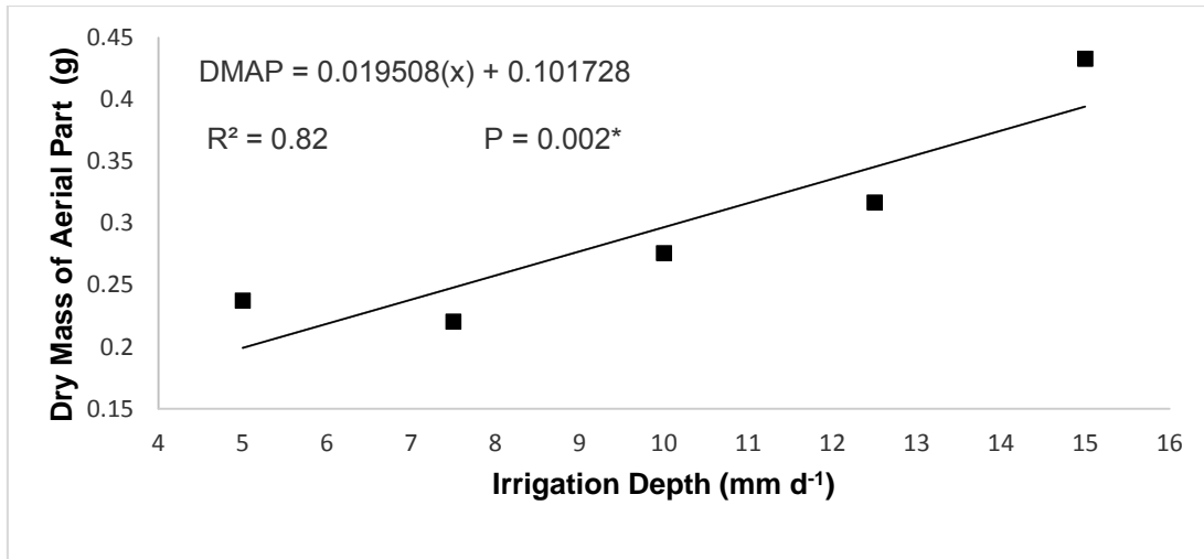
Fig. 3. Estimating the collecting dry mass of aerial part (DMAP) of conilon coffee seedlings as a function of the irrigation depth.
