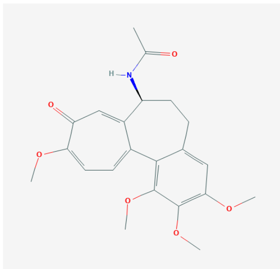
Figure 1. Chemical structure of Colchicine (Source from PubChem.)
