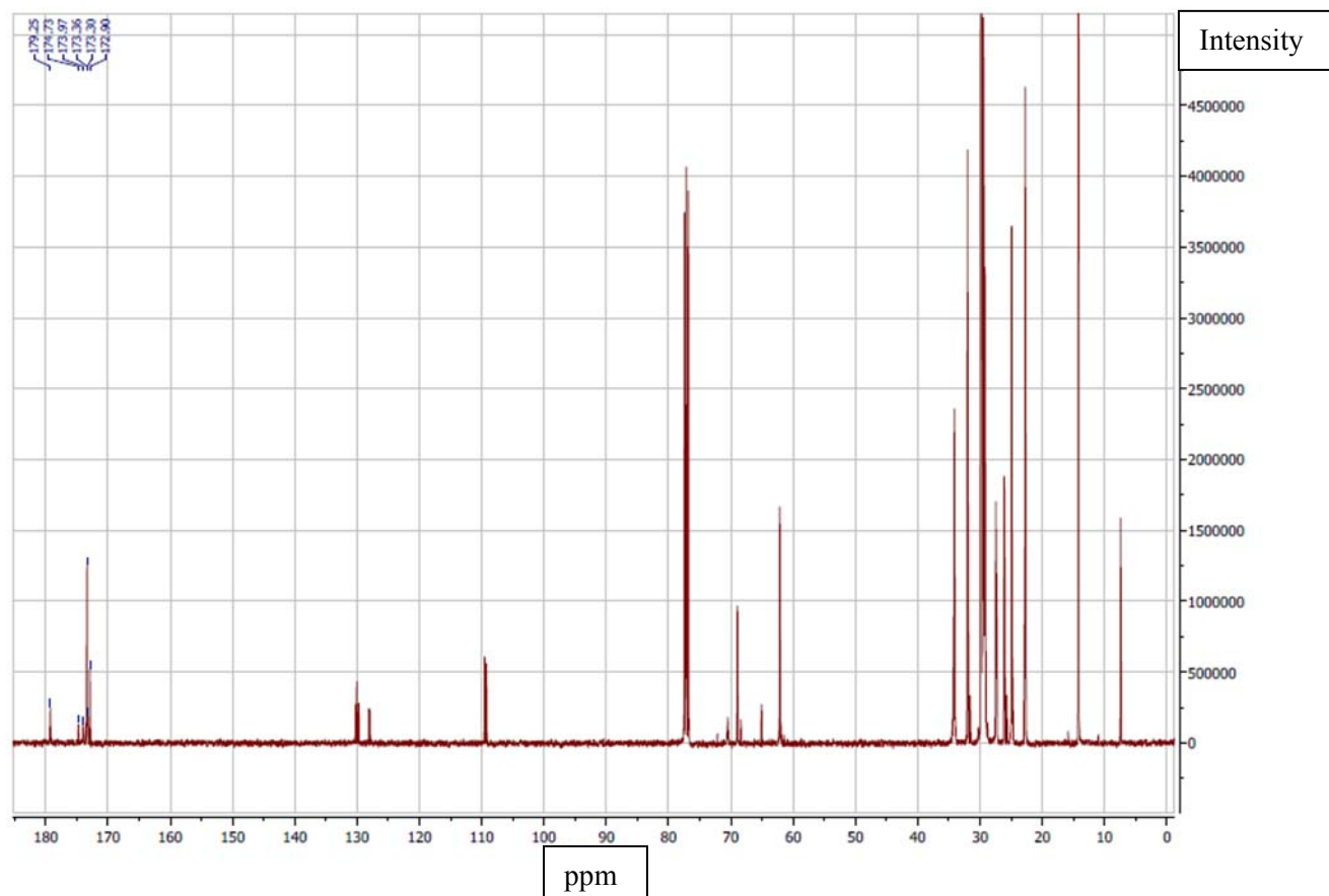
Figure 4: ^{13}\text{C} -NMR spectrum of Pachira aquatica seed oil.
