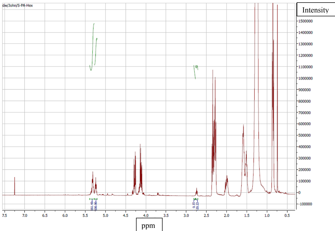
Figure 2: ^1\text{H} NMR spectrum of Pachira aquatica seed oil.
