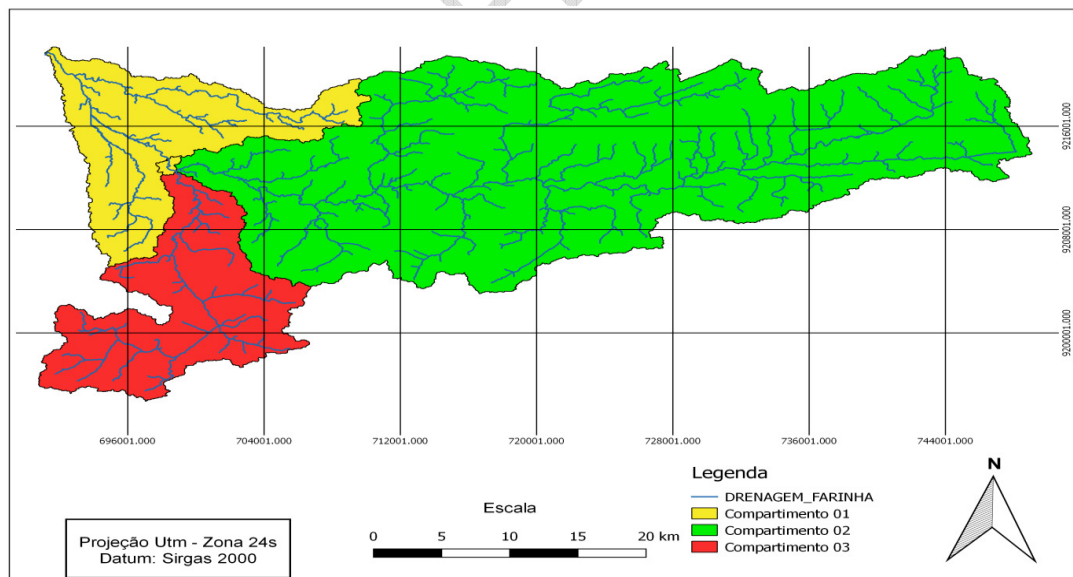
Figure 3. Map of compartmentalization and drainage of the river basin of Farinha-PB.
