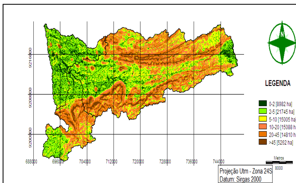
Figure 4- Slope map of the River Farinha micro-basin
