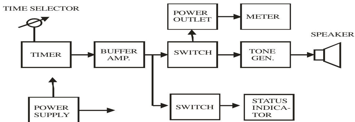
Figure 1: Block Diagram of the Cooker Control Unit
