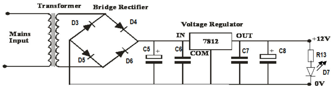
Figure 8: Power Supply Unit
