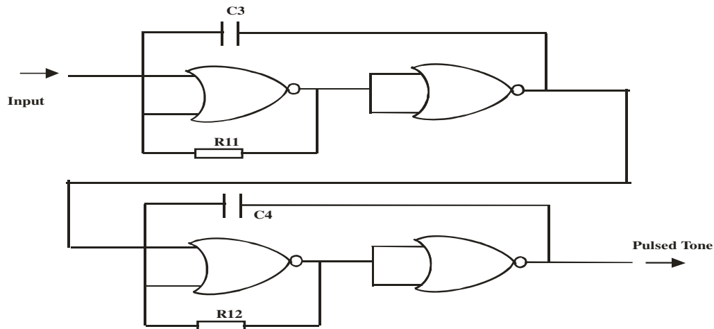
Figure 5: NOR Gates Configuration
