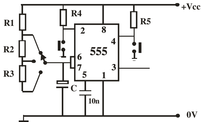
Figure 2: The Timer Showing Timing Resistors
