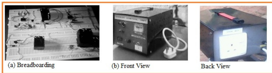
Figure 9: The Cooker Control Unit showing Components Wiring on Breadboard and its Completed Front and Back View
