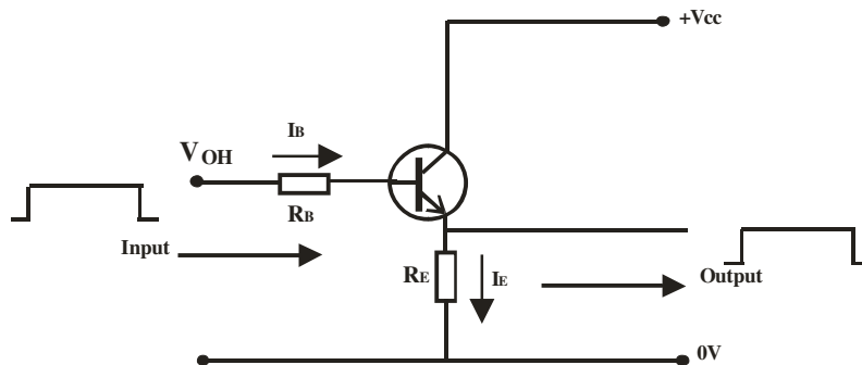
Figure 3: A Common Collector Amplifier Serving as a Buffer
