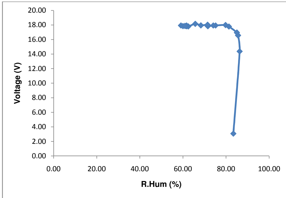
Fig. 5: Voltage (V) against relative humidity (%)
