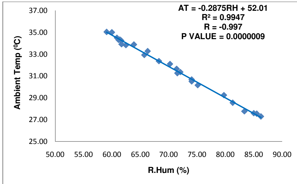
Fig. 3: Ambient temperature (°C) against relative humidity (%)
