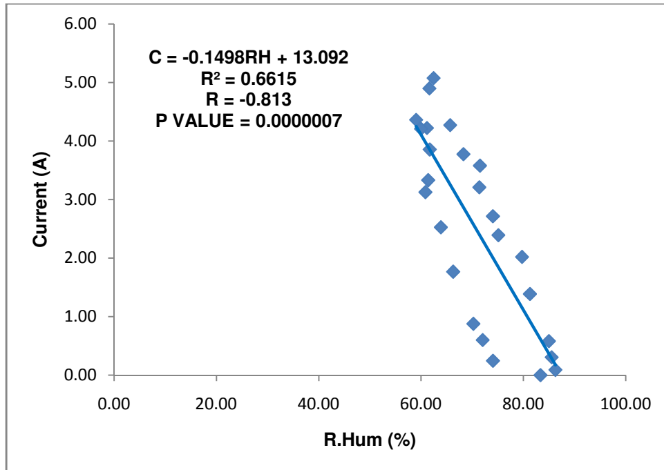
Fig. 6: Current (A) against relative humidity (%)
