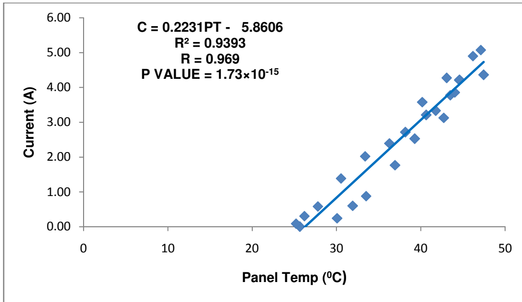
Fig. 9: Current (A) against panel temperature (°C)
