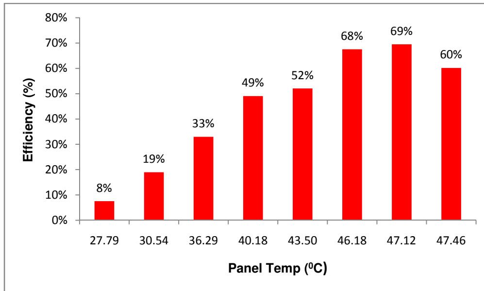
Fig. 10: Efficiency (%) against panel temperature (°C)
