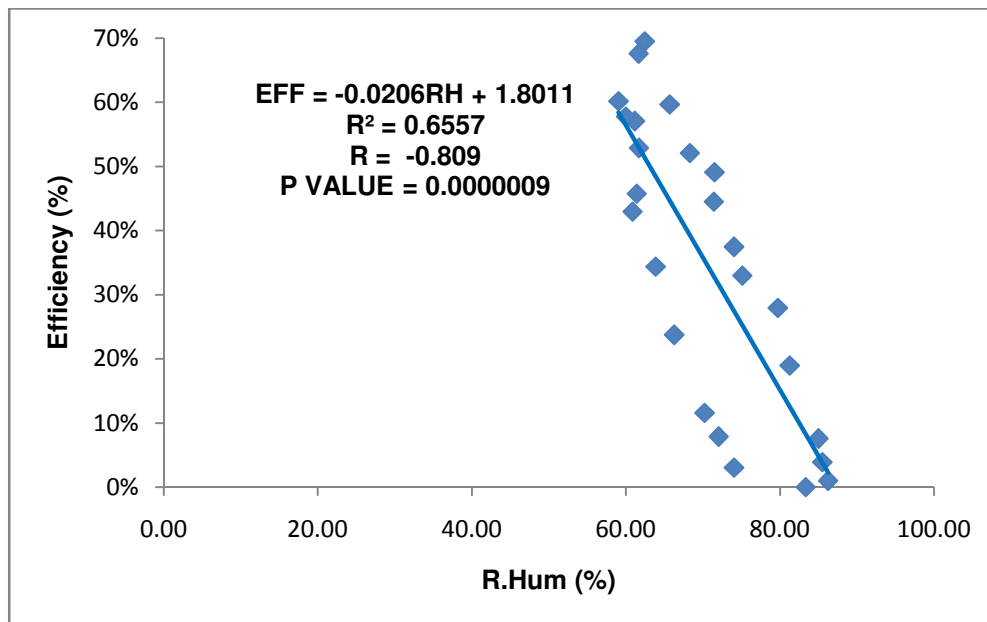
Fig. 7: Efficiency (%) against relative humidity (%)
