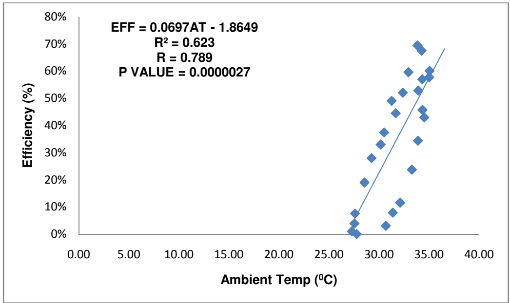
Fig. 11: Efficiency (%) against ambient temperature (°C)
