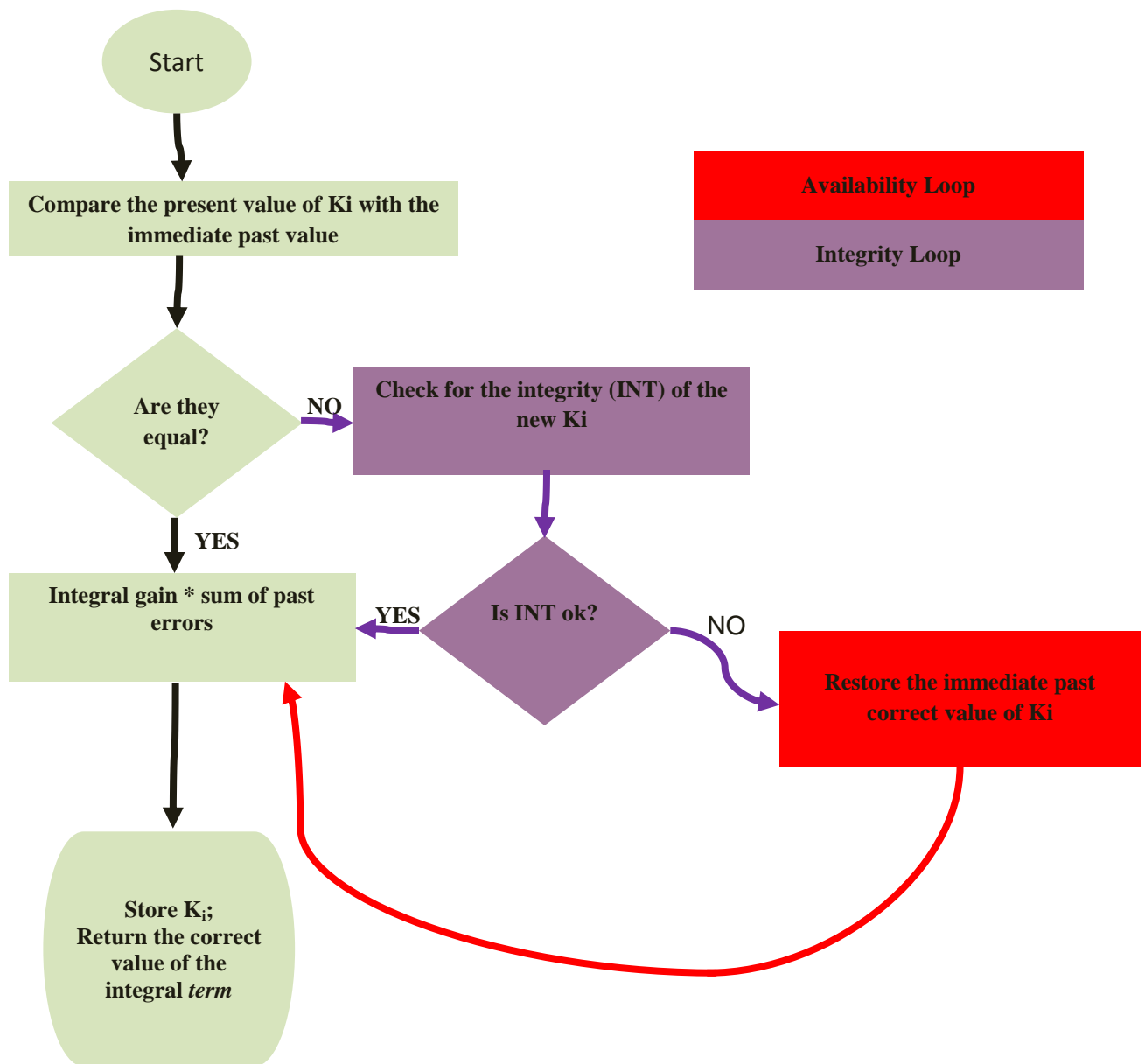
Fig. 14. High level flow chart for calculation of secure integral term in a PID control loop
