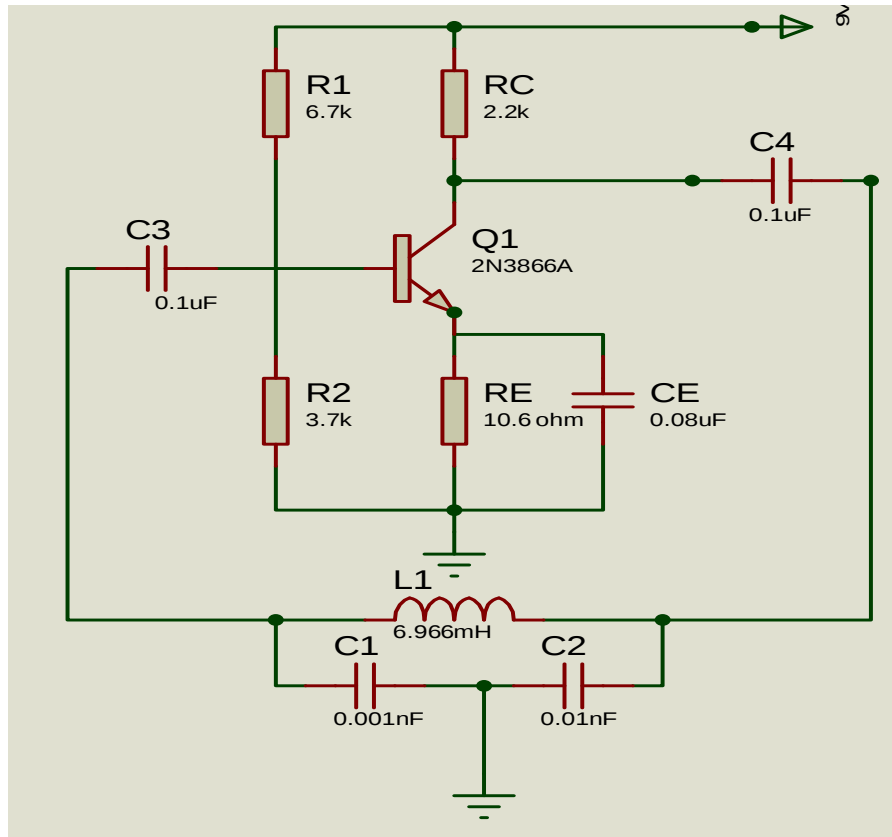
Figure 2: Designed Colpitt's Oscillator
