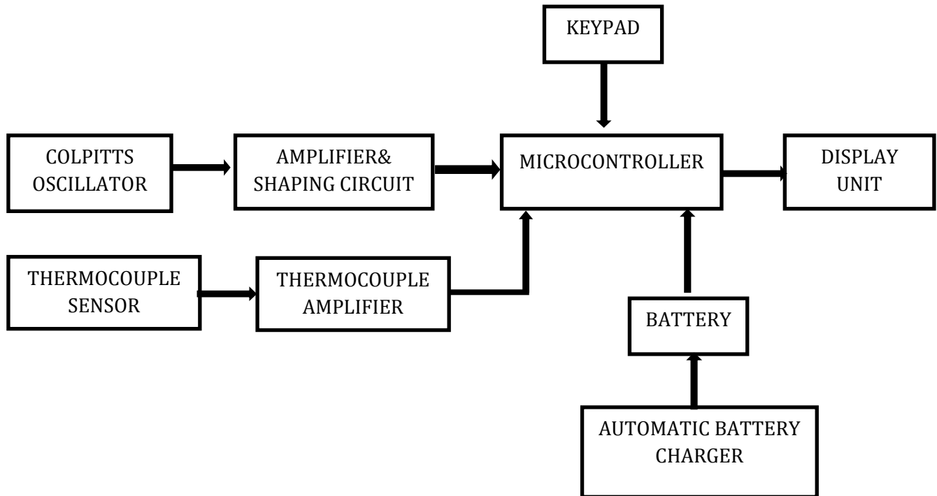
Figure 1: Proposed Block Diagram of the ParamagnetismAnalyser
