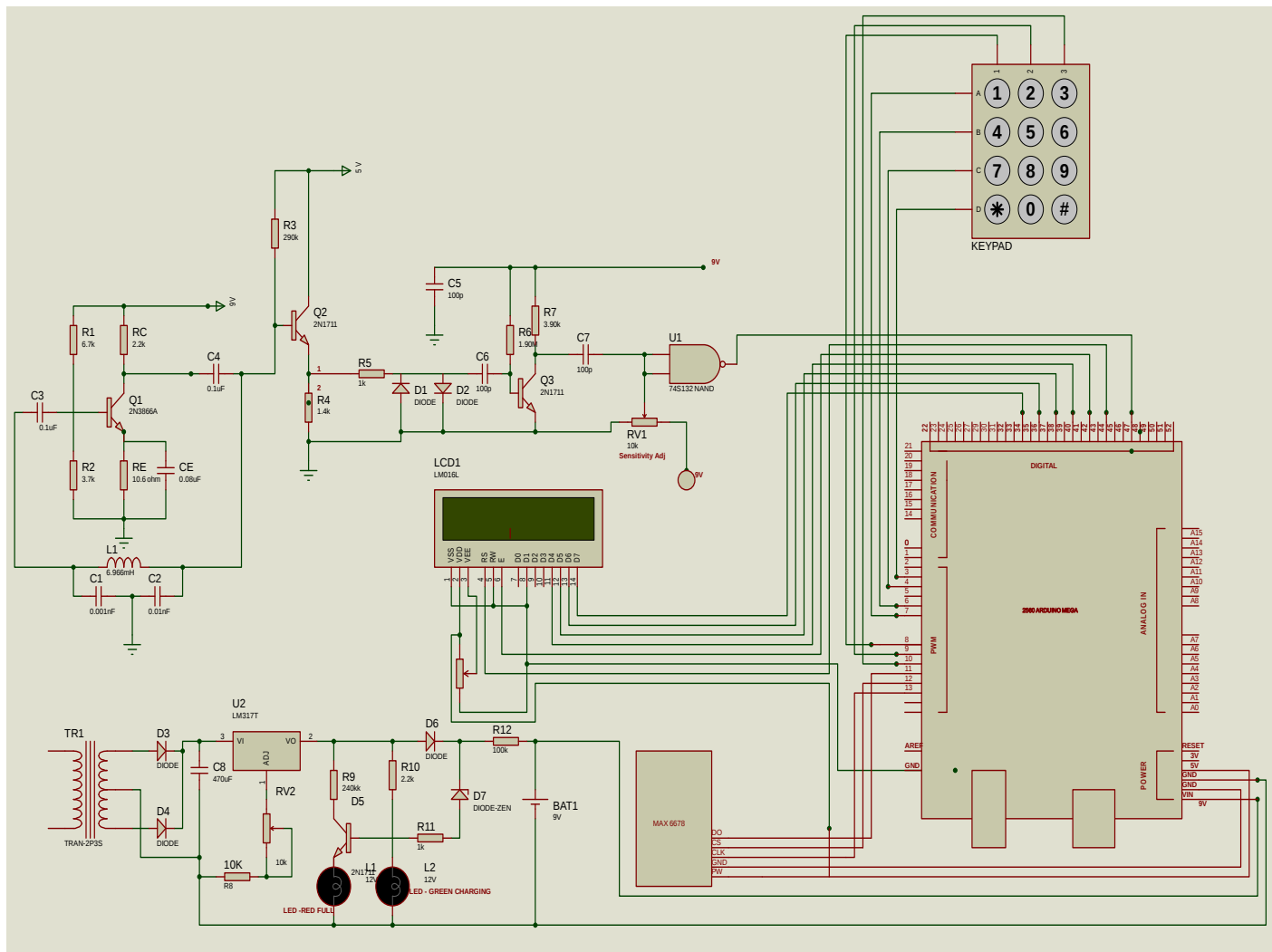
Figure 5: Complete Circuit Diagram of the Developed ParamagnetismAnalyser.
