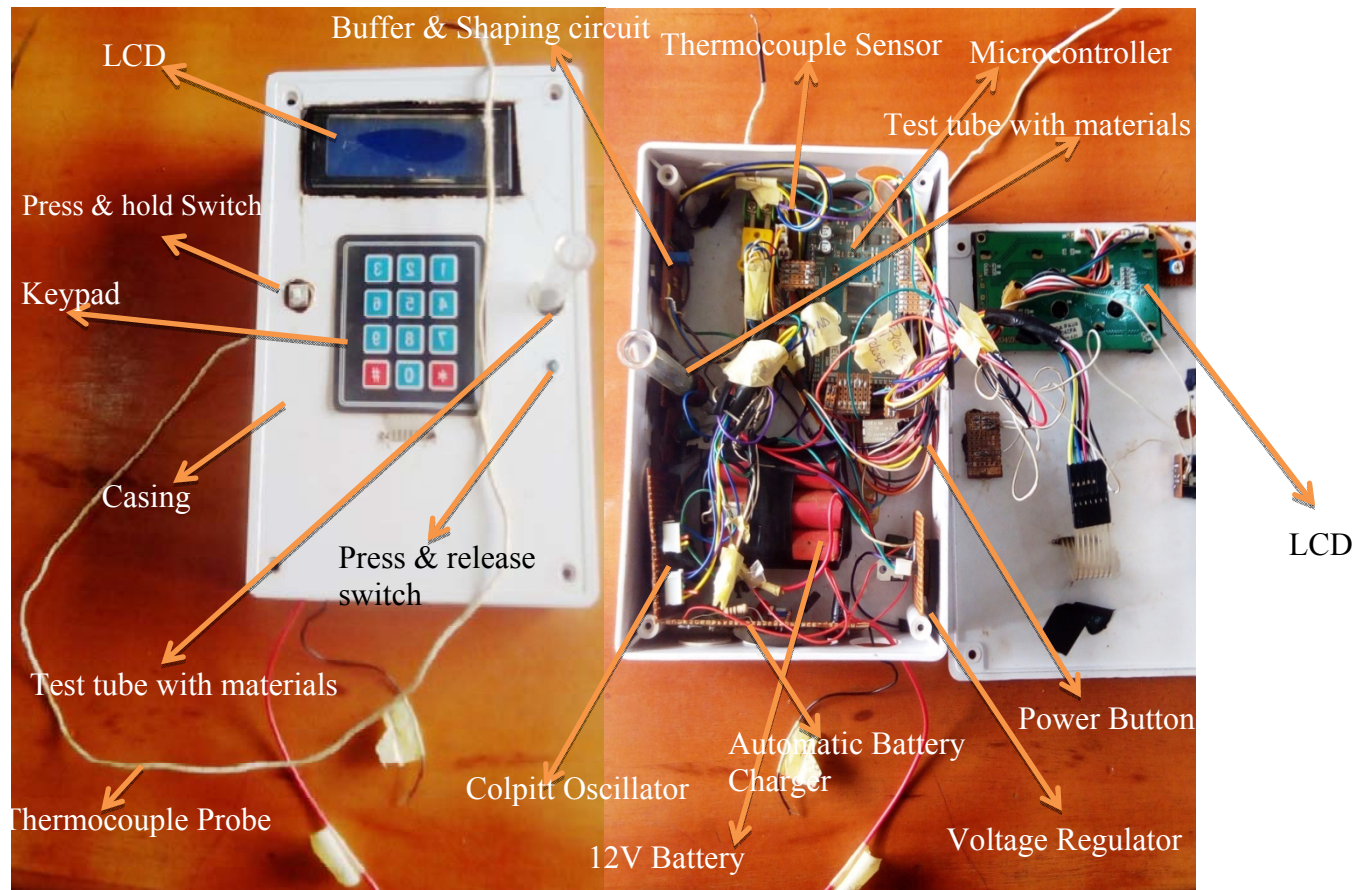
Figure 6: Image of the developed Paramagnetism Analyzer
