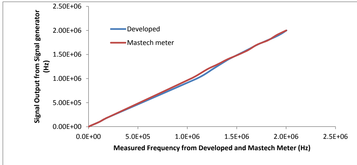
Figure 7: Comparative plot of developed Frequency Counter against Standard Frequency meter with respect to a varying signal generator.
