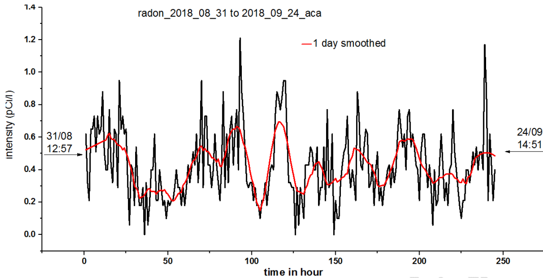
Fig. 8 - Radon gas measurements in ACA Tower from 31/08 to 24/09 of 2018.
