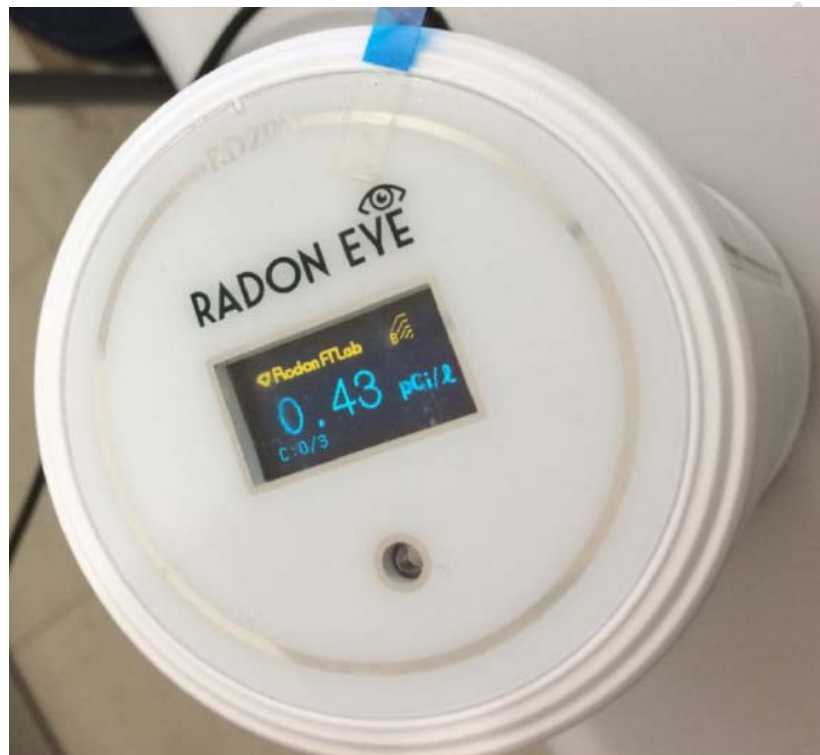
Fig 3 – Top view of Radon Eye RD200 ionization chamber used for monitoring radon gas [11]
