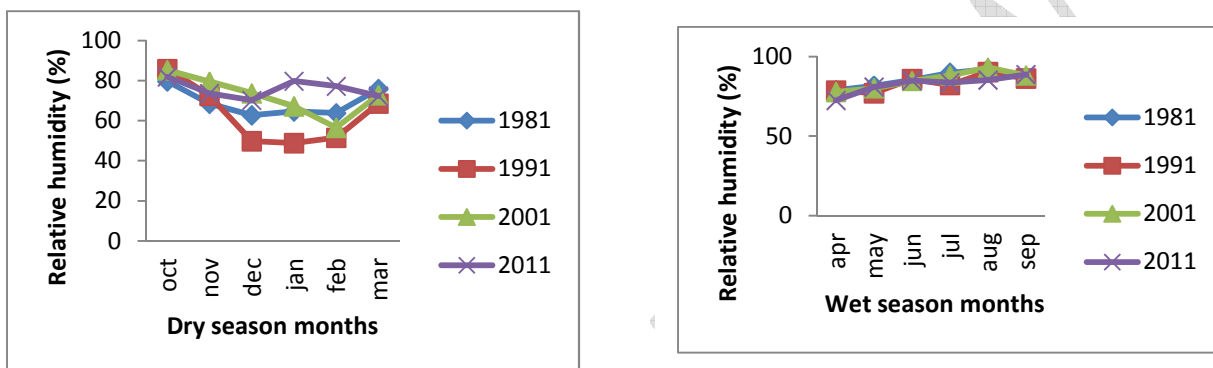
Figure 2 (b) Seasonal patterns for (i) dry season months and (ii) wet season months for Relative humidity in Calabar
