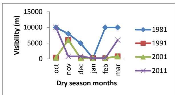
Figure 6 (a) Seasonal patterns for (i) dry season months and (ii) wet season months for Visibility in Warri.
