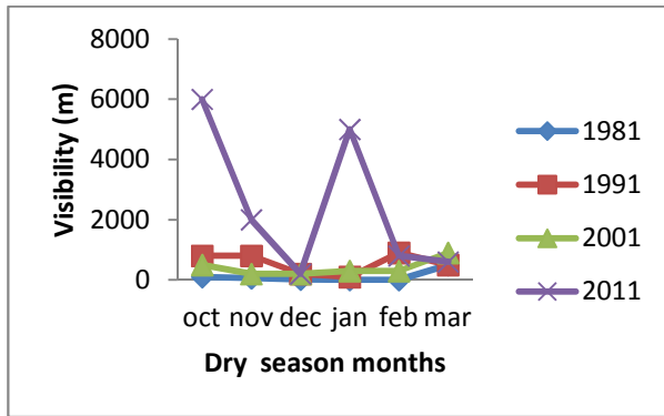
Figure 9 (a) Seasonal patterns for (i) dry season months and (ii) wet season months for Visibility in Uyo
