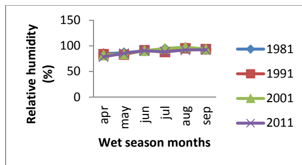
Figure 5 (b) Seasonal patterns for (i) dry season months and (ii) wet season months for Relative humidity in Owerri.
