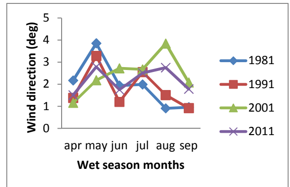
Figure 12. (b) Seasonal patterns for (i) dry season months and (ii) wet season months for Wind direction in Warri.
