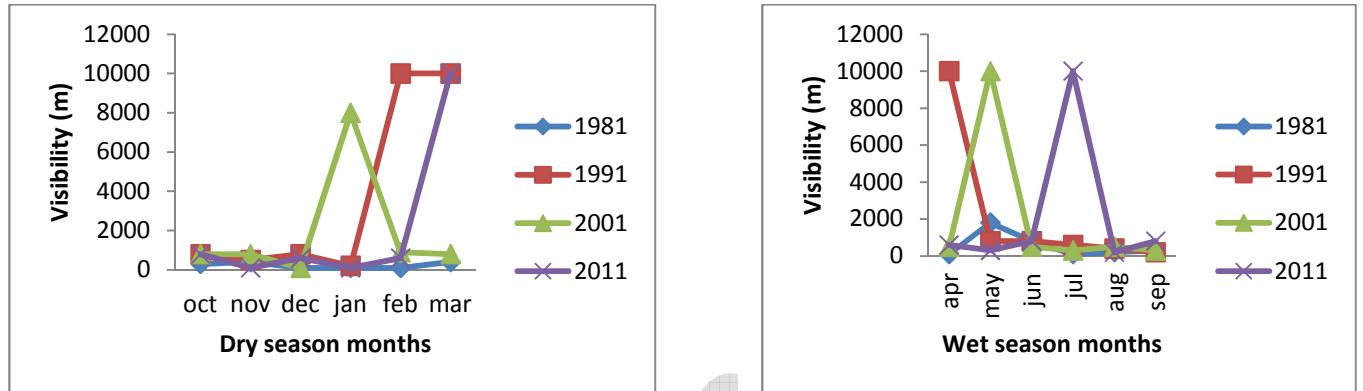
Figure 8 (a) Seasonal patterns for (i) dry season months and (ii) wet season months for Visibility in Calabar.
