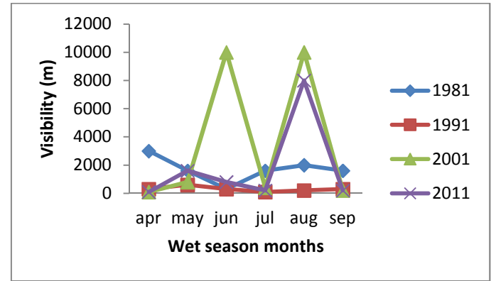
Figure 10. (a) Seasonal patterns for (i) dry season months and (ii) wet season months for Visibility in Port harcourt.
