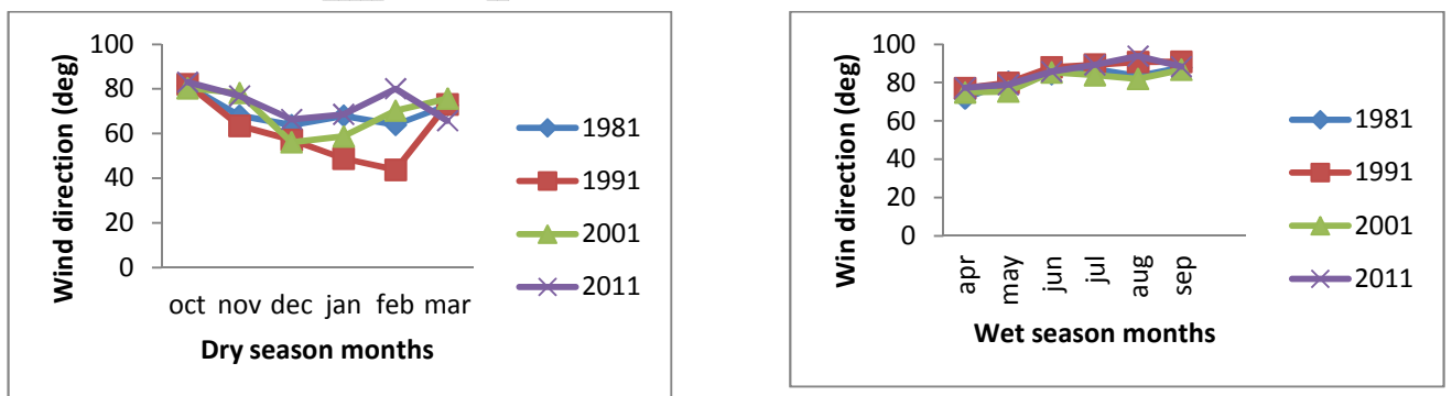
Figure 8. (b) Seasonal patterns for (i) dry season months and (ii) wet season months for Wind direction in Calabar.
