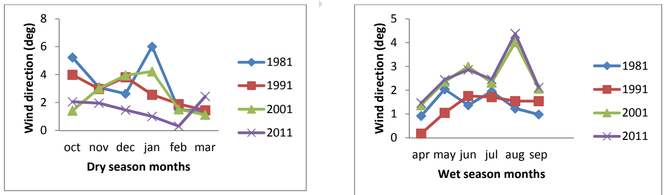
Figure 13. (b) Seasonal patterns for (i) dry season months and (ii) wet season months for Wind direction in Akure.
