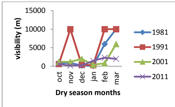
Figure7 (a) Seasonal patterns for (i) dry season months and (ii) wet season months for Visibility in Akure.
