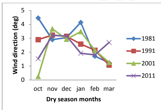
Figure 11. (b) Seasonal patterns for (i) dry season months and (ii) wet season months for Wind direction in Owerri.
