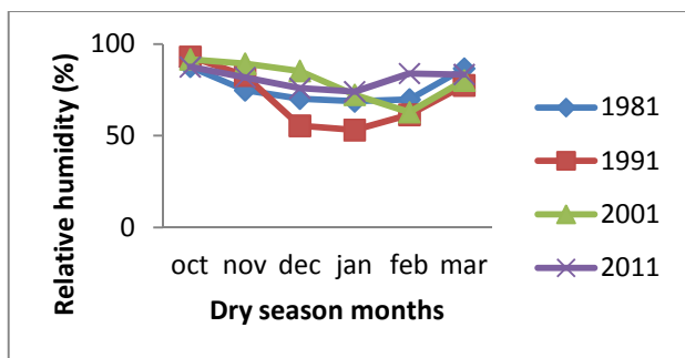
Figure 5 (b) Seasonal patterns for (i) dry season months and (ii) wet season months for Relative humidity in Owerri.
