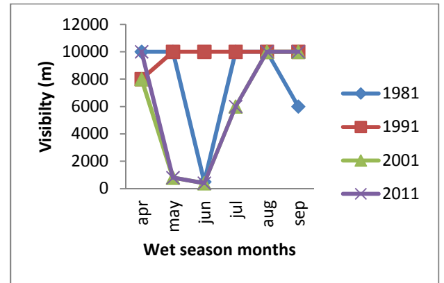
Figure 12. (a) Seasonal patterns for (i) dry season months and (ii) wet season months for Visibility in Warri.
