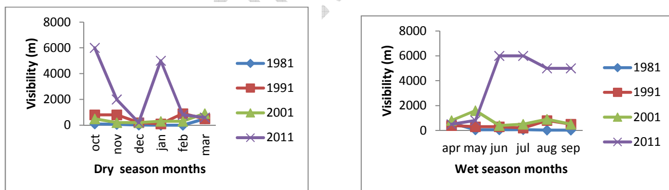
Figure 3 (a) Seasonal patterns for (i) dry season months and (ii) wet season months for Visibility in Uyo.
