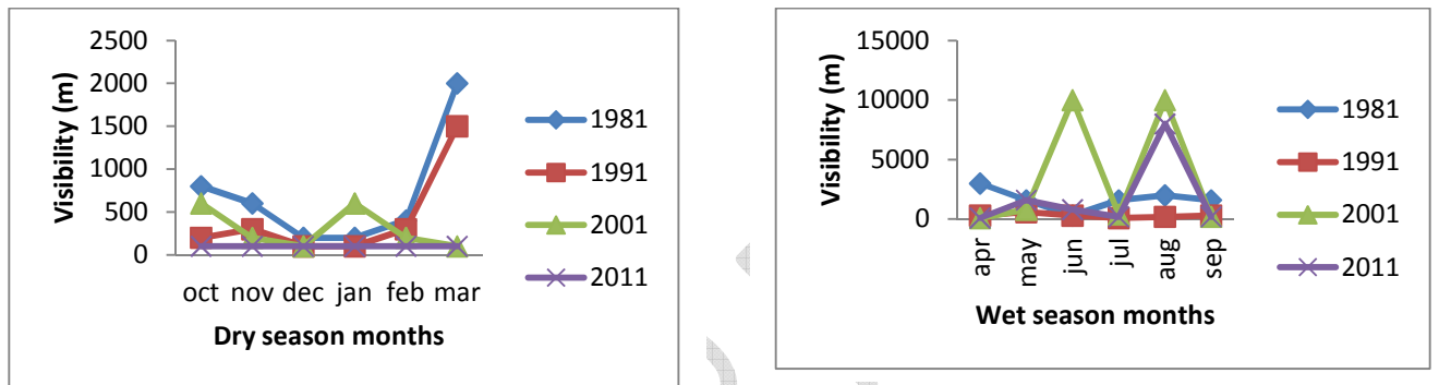
Figure 4 (a) Seasonal patterns for (i) dry season months and (ii) wet season months for Visibility in Port harcourt.
