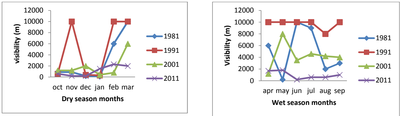
Figure 13. (a) Seasonal patterns for (i) dry season months and (ii) wet season months for Visibility in Akure.
