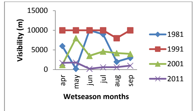
Figure7 (a) Seasonal patterns for (i) dry season months and (ii) wet season months for Visibility in Akure.
