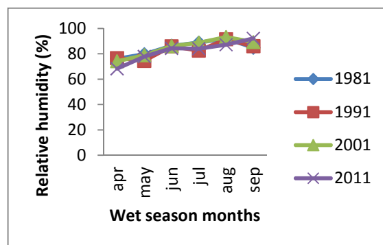
Figure 6. (b) Seasonal patterns for (i) dry season months and (ii) wet season months for Relative humidity in Warri.
