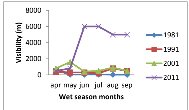
Figure 9 (a) Seasonal patterns for (i) dry season months and (ii) wet season months for Visibility in Uyo
