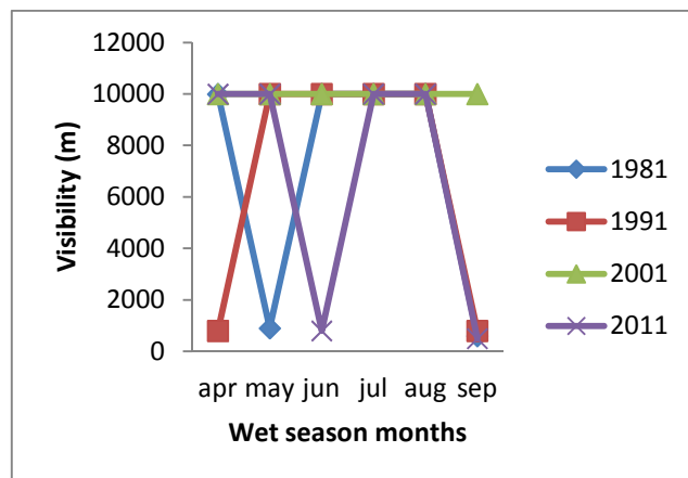
Figure 11. (a) Seasonal patterns for (i) dry season months and (ii) wet season months for Visibility in Owerri.
