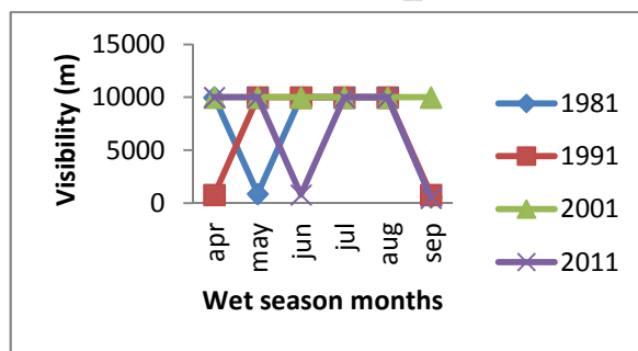
Figure 5 (a) Seasonal patterns for (i) dry season months and (ii) wet season months for Visibility in Owerri.
