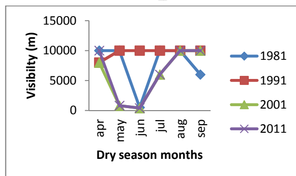
Figure 6 (a) Seasonal patterns for (i) dry season months and (ii) wet season months for Visibility in Warri.
