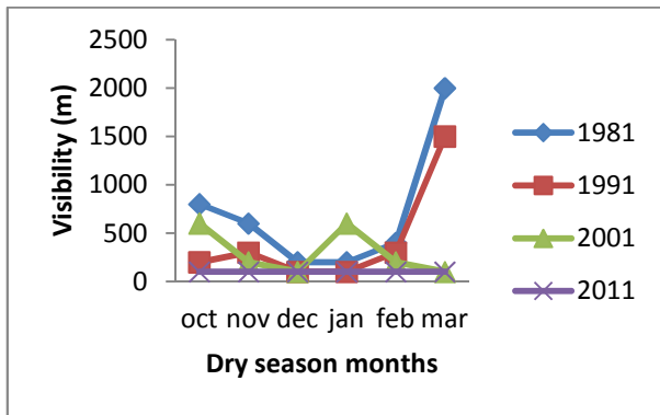
Figure 10. (a) Seasonal patterns for (i) dry season months and (ii) wet season months for Visibility in Port harcourt.
