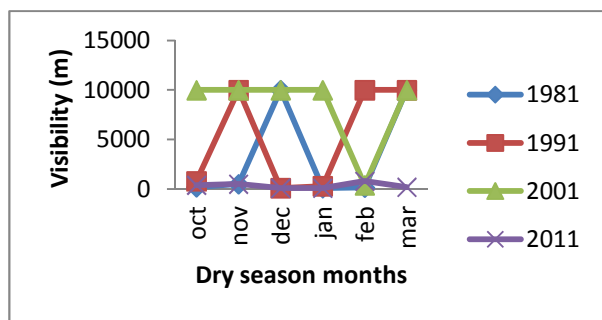
Figure 5 (a) Seasonal patterns for (i) dry season months and (ii) wet season months for Visibility in Owerri.
