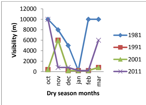
Figure 12. (a) Seasonal patterns for (i) dry season months and (ii) wet season months for Visibility in Warri.
