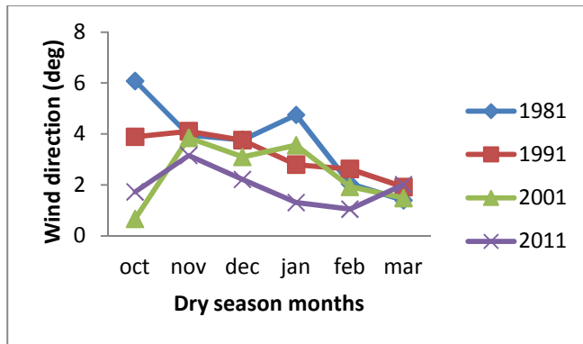
Figure 12. (b) Seasonal patterns for (i) dry season months and (ii) wet season months for Wind direction in Warri.
