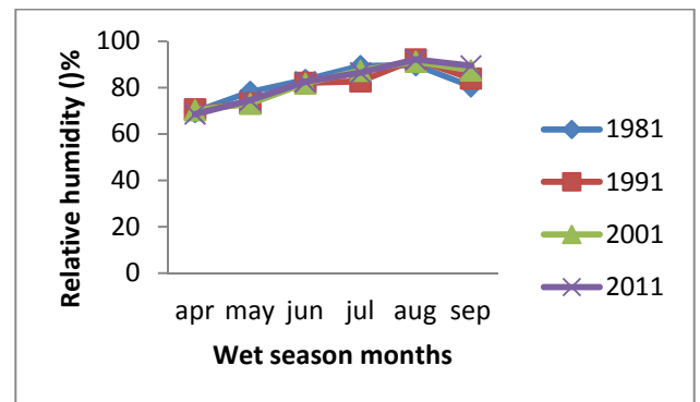
Figure 7 (b) Seasonal patterns for (i) dry season months and (ii) wet season months for Relative humidity in Akure.
