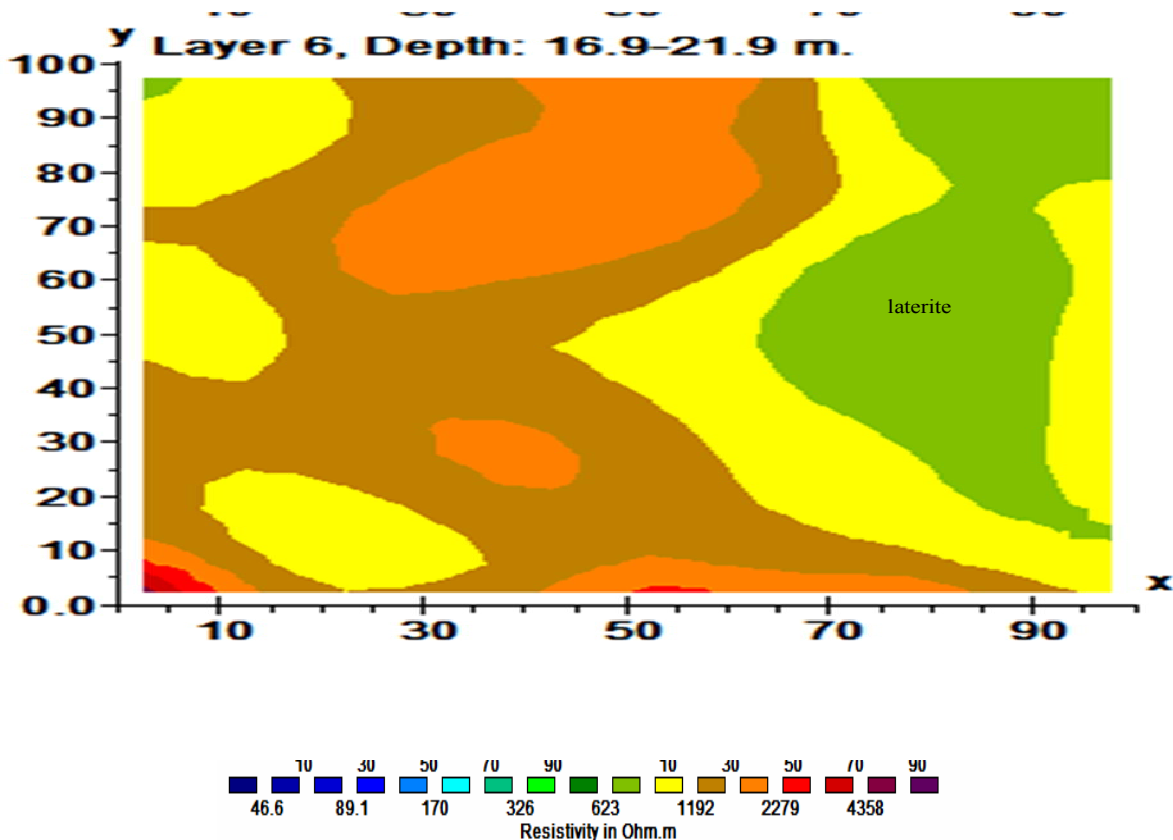
Figure 8: A 3-D resistivity inversion slice along x-y coordinates at a depth of (16.90 - 21.90m).
