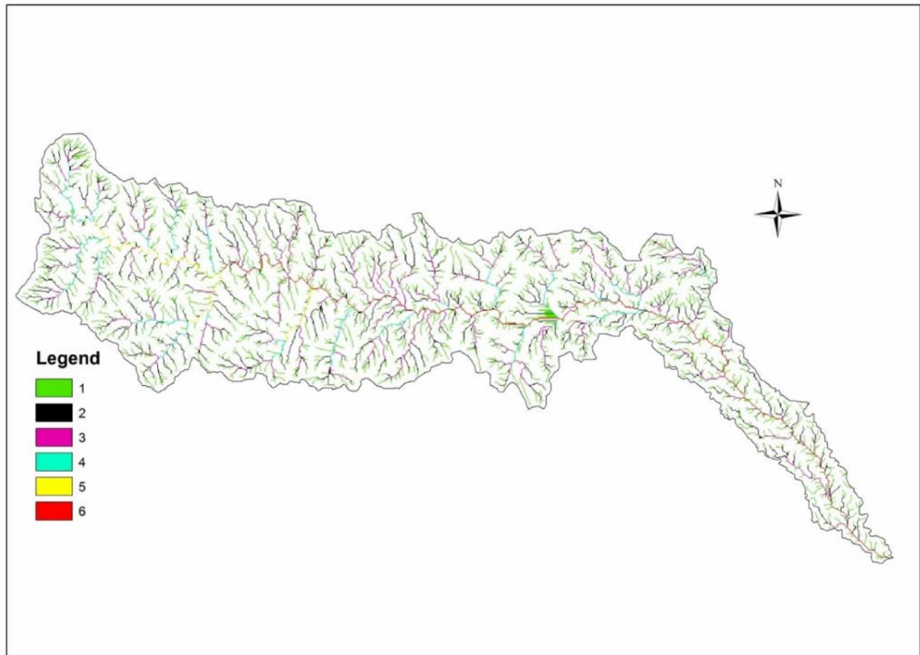
Figure 2 Stream order of the Adula watershed
