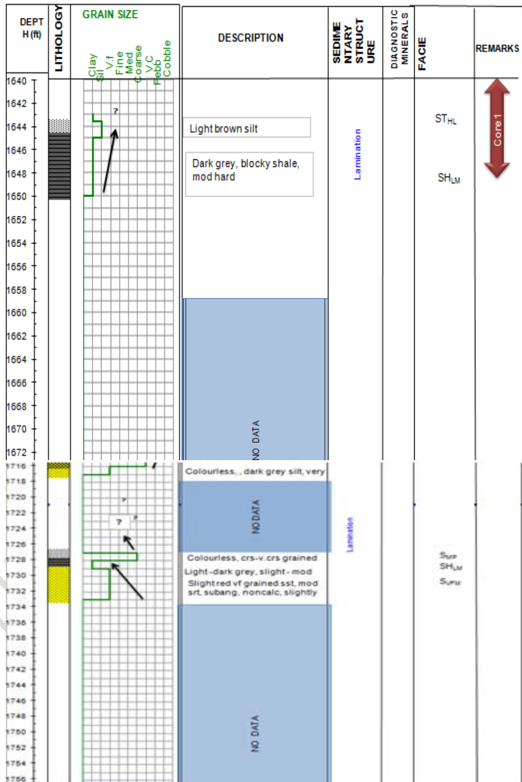
Figure 6: Lithology Log of 'Valz-01' well
