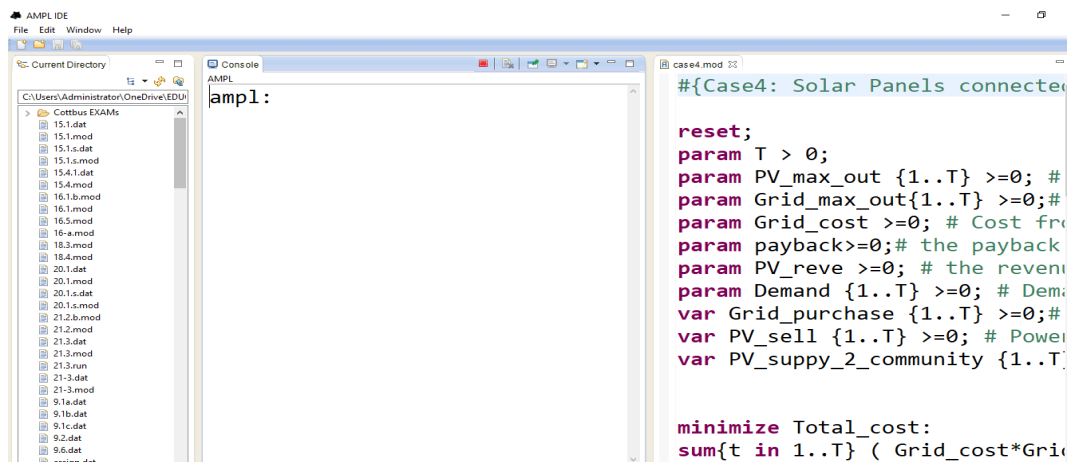
Figure 3: AMPL interface.
