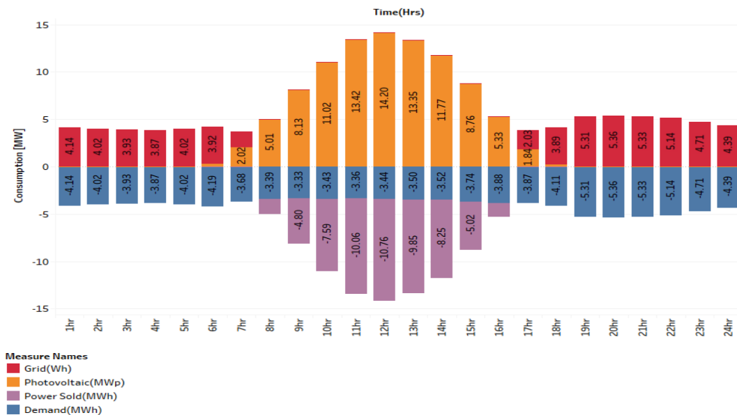
Figure 7: A graph showing the power scheduling for scenario 2
