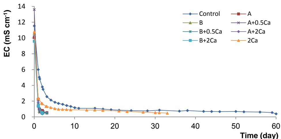
Fig. 2. Periodical change of EC in the eluents from soil columns
