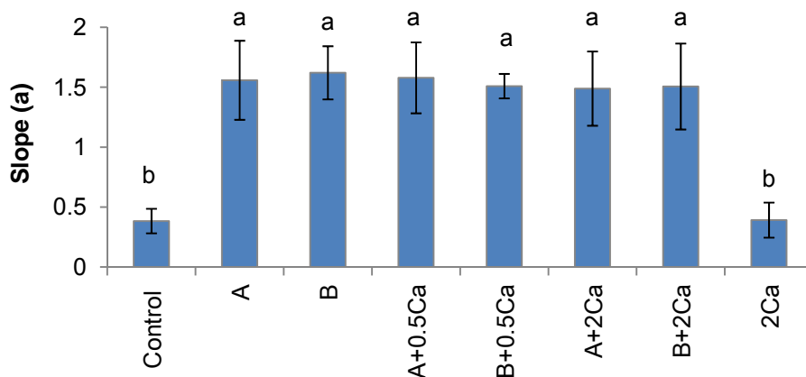
Fig. 1. Comparison of slope values in the infiltration rates from 24 to 48 hours
