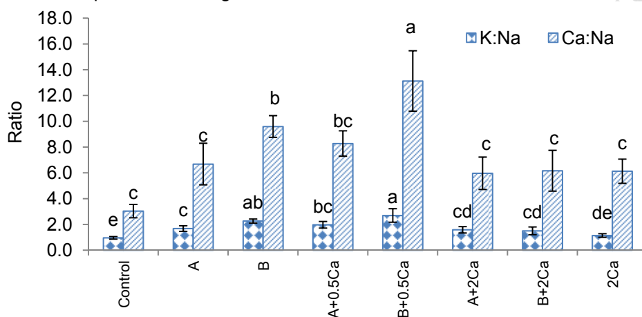
Fig. 6. Ratio of exchangeable K/Na and exchangeable Ca/Na of soil after leaching Difference letters indicate significant differences (Fisher test, P = .05 ) among treatments. Bars represent standard deviation
