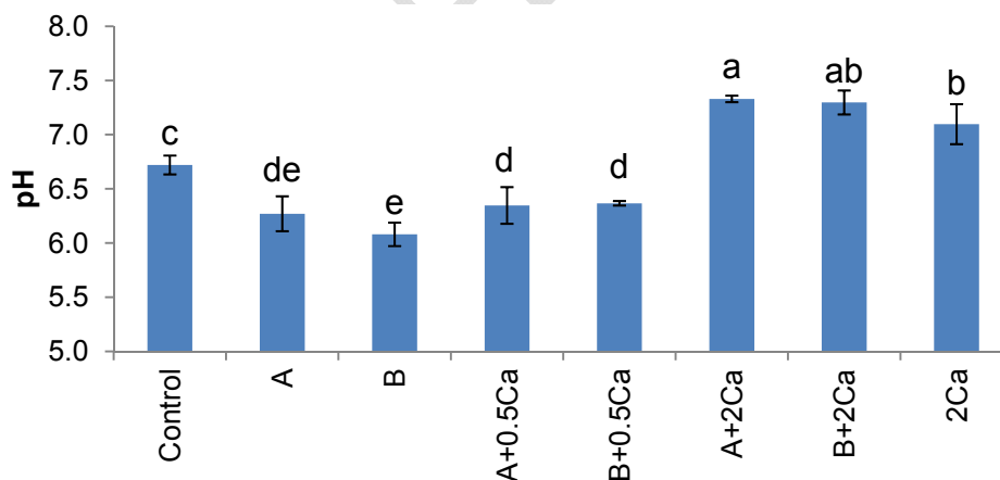
Fig. 3. pH (H 2 O) of soil after leaching
