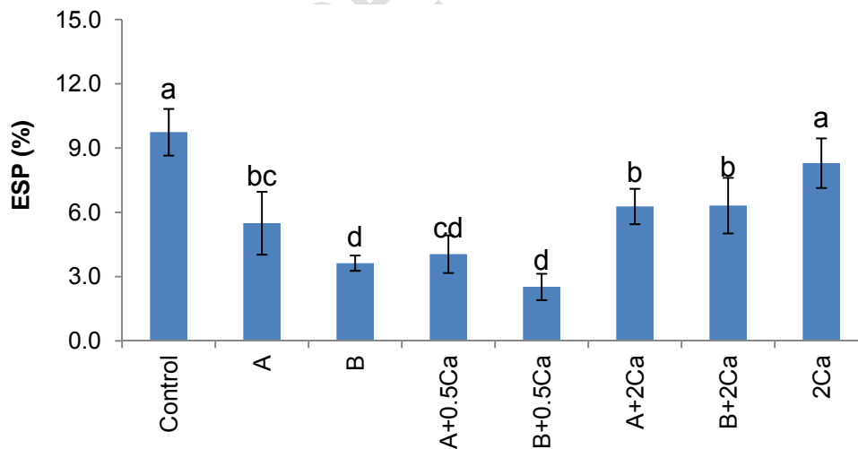
Fig. 5. Exchangeable Sodium Percentage (ESP) of soil after leaching
