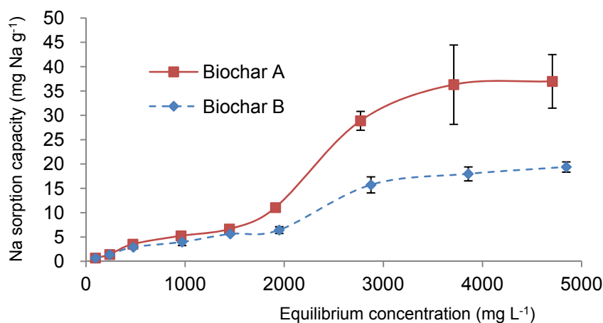
Fig. 7. Sorption isotherm of Na + on two different biochars ( P < .001 ). Bars represent standard deviation of n = 4 .
