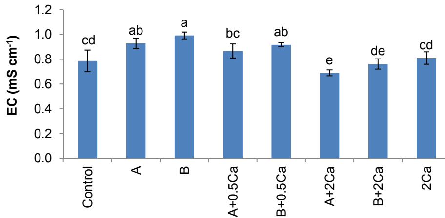
Fig. 4. EC of soil after leaching
