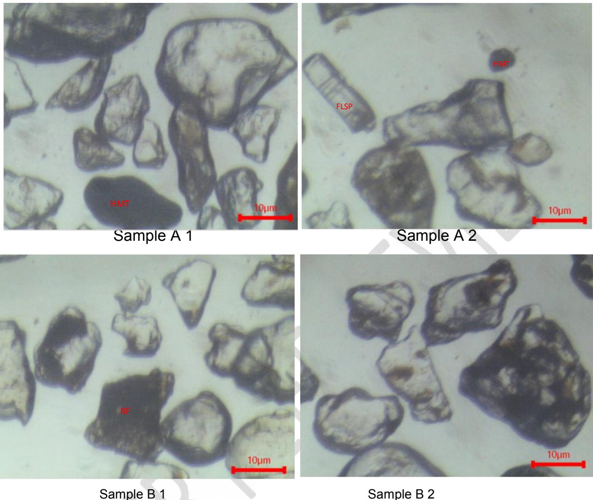
Fig. 6: Photomicrograph of grains in sample A and B showing types of shapes, dominance of quartz grains, and rare presence of rock fragments (RF), reniform or kidney shaped hematite (HM) and prismatic feldspar (FLSP) grains.
