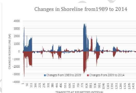
Figure 5: Total Shoreline profile changes from 1989 to 2014
