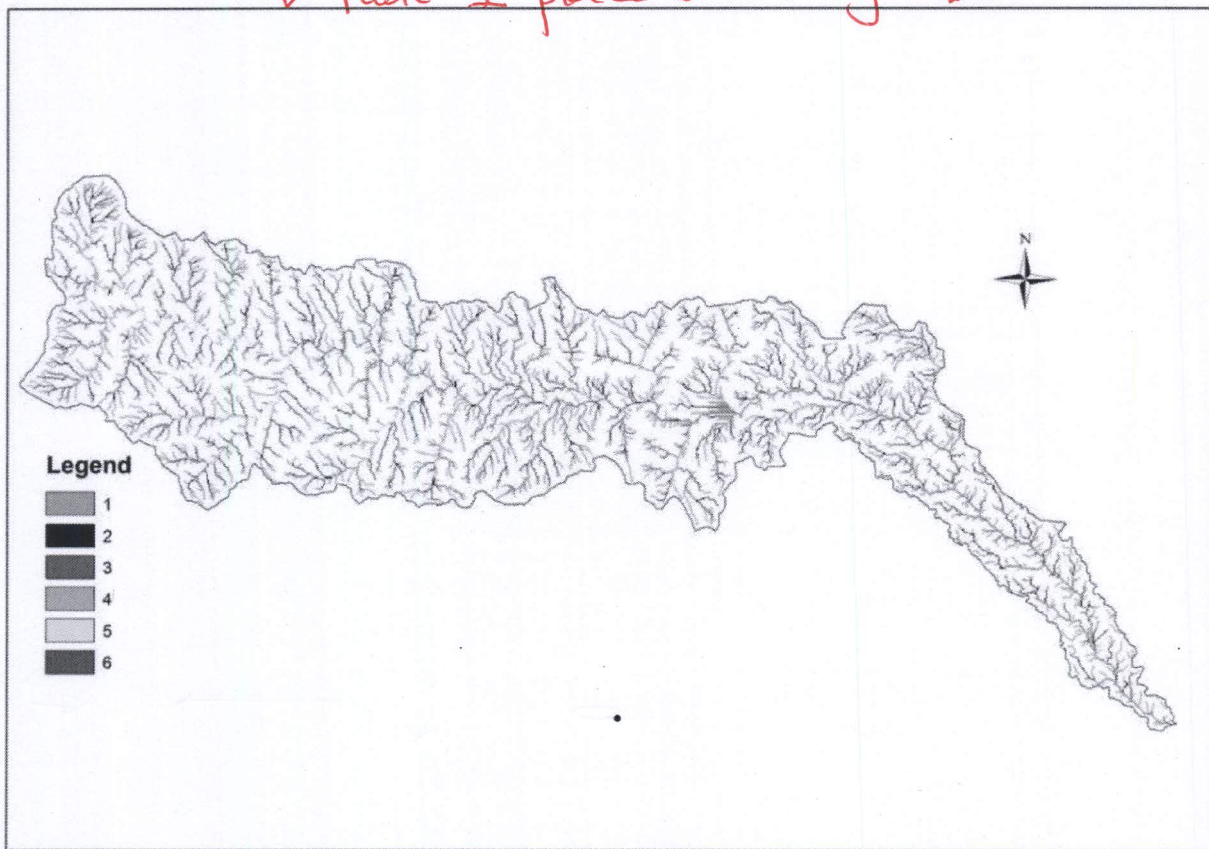
Figure 2 Stream order of the Adula watershed
