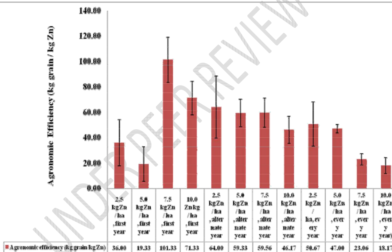
Fig. 1 Agronomic efficiency (kg grain/kg Zn) of the different Zn treatments in rice during fourth year under rice-wheat cropping system
